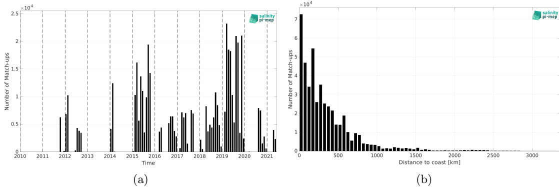
Figure 2: Number of match-ups between TSG (GOSUD-Research-vessel) and SMOS SSS L3 v2 - 9-Days (BEC) SSS as a function of time (a) and as function of the distance to coast (b) over the South Pacific Ocean Pi-MEP region and for the full satellite product period.
