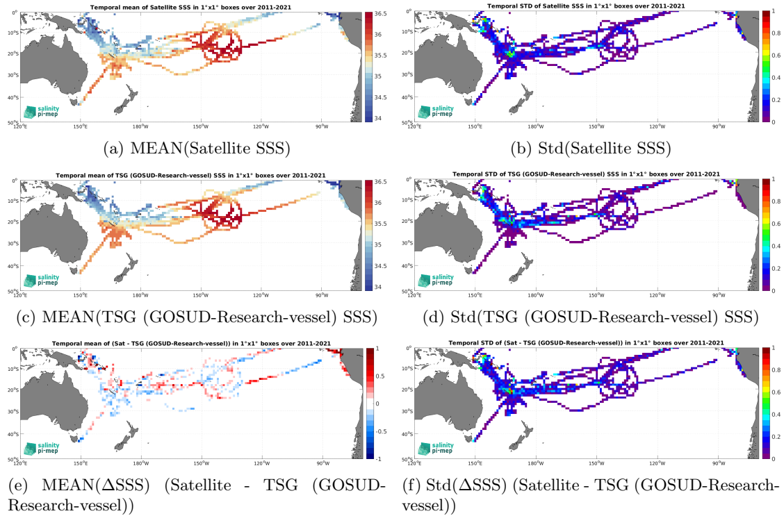
Figure 7: Temporal mean (left) and Std (right) of SSS from SMOS SSS L3 v2 - 9-Days (BEC) (top), TSG (GOSUD-Research-vessel) (middle), and of \Delta SSS (Satellite - TSG (GOSUD-Research-vessel)). Only match-up pairs are used to generate these maps.
