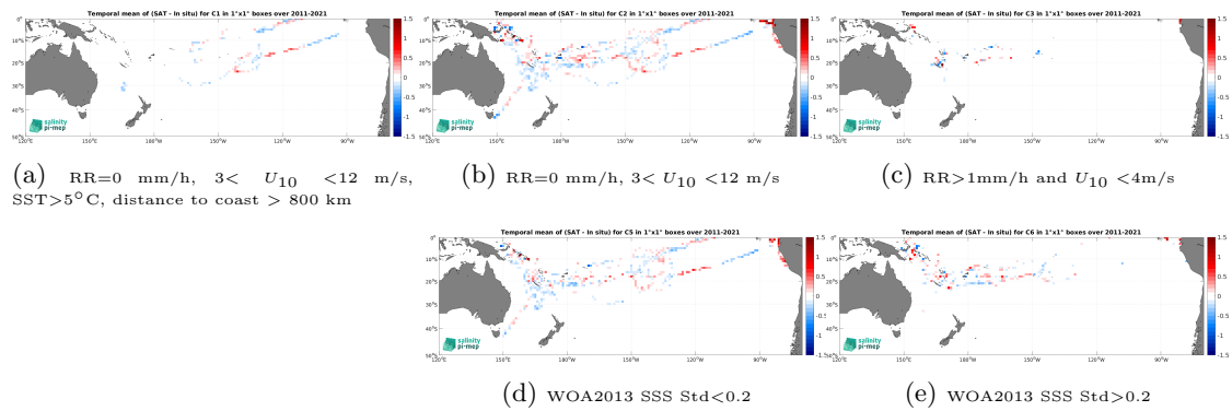
Figure 14: Temporal mean gridded over spatial boxes of size 1^\circ \times 1^\circ of \Delta SSS (SMOS SSS L3 v2 - 9-Days (BEC) - TSG (GOSUD-Research-vessel)) for 5 different subdatasets corresponding to:RR=0 mm/h, 3 < U_{10} < 12 m/s, SST >5^\circ\text{C} , distance to coast > 800 km (a), RR=0 mm/h, 3 < U_{10} < 12 m/s (b), RR >1 mm/h and U_{10} < 4 m/s (c), WOA2013 SSS Std <0.2 (d), WOA2013 SSS Std >0.2 (e).
