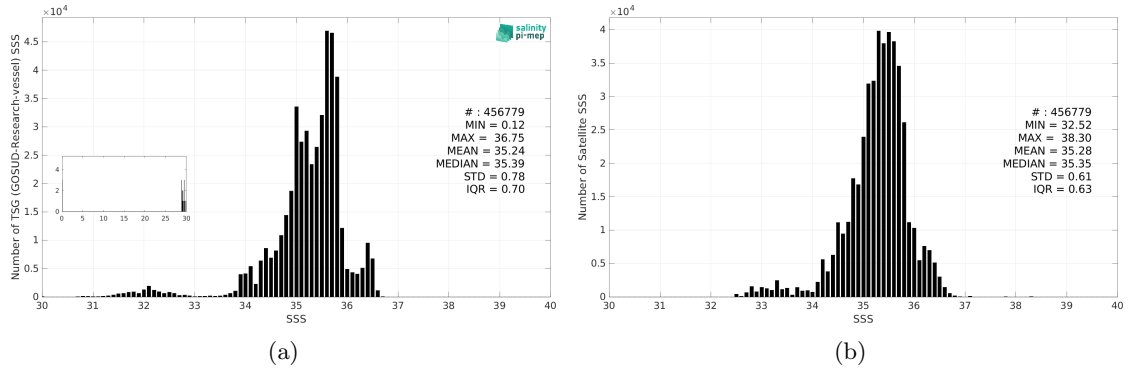
Figure 3: Histograms of SSS from TSG (GOSUD-Research-vessel) (a) and SMOS SSS L3 v2 - 9-Days (BEC) (b) considering all match-up pairs per bins of 0.1 over the South Pacific Ocean Pi-MEP region and for the full satellite product period.
