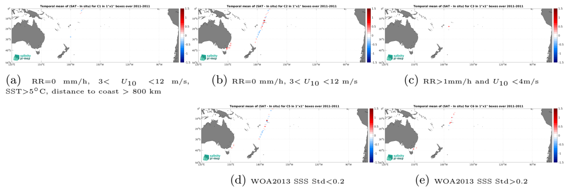
Figure 14: Temporal mean gridded over spatial boxes of size 1^\circ \times 1^\circ of \Delta SSS (SMOS SSS L3 v2 - 9-Days (BEC) - TSG (CSIC-UTM)) for 5 different subdatasets corresponding to:RR=0 mm/h, 3 < U_{10} < 12 m/s, SST>5°C, distance to coast > 800 km (a), RR=0 mm/h, 3 < U_{10} < 12 m/s (b), RR>1mm/h and U_{10} < 4 m/s (c), WOA2013 SSS Std<0.2 (d), WOA2013 SSS Std>0.2 (e).
