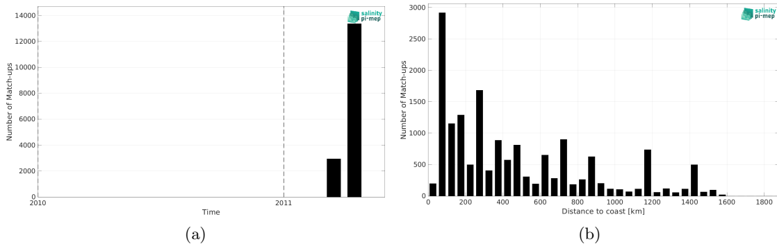
Figure 2: Number of match-ups between TSG (CSIC-UTM) and SMOS SSS L3 v2 - 9-Days (BEC) SSS as a function of time (a) and as function of the distance to coast (b) over the South Pacific Ocean Pi-MEP region and for the full satellite product period.
