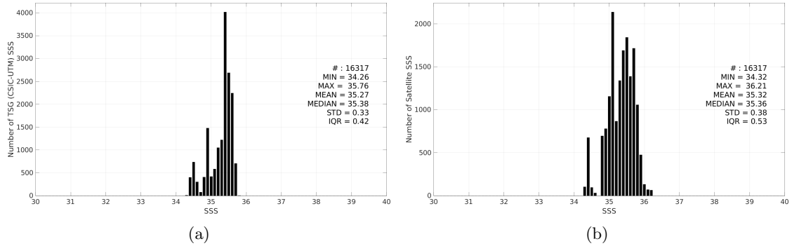
Figure 3: Histograms of SSS from TSG (CSIC-UTM) (a) and SMOS SSS L3 v2 - 9-Days (BEC) (b) considering all match-up pairs per bins of 0.1 over the South Pacific Ocean Pi-MEP region and for the full satellite product period.
