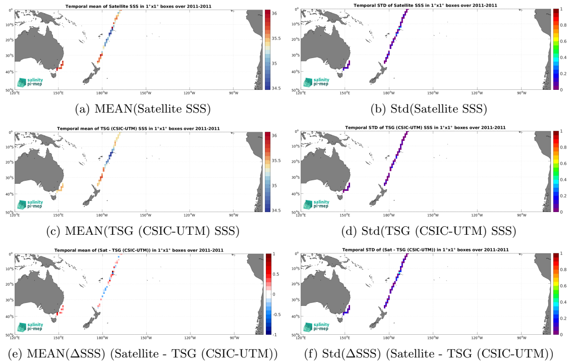
Figure 7: Temporal mean (left) and Std (right) of SSS from SMOS SSS L3 v2 - 9-Days (BEC) (top), TSG (CSIC-UTM) (middle), and of \Delta SSS (Satellite - TSG (CSIC-UTM)). Only match-up pairs are used to generate these maps.
