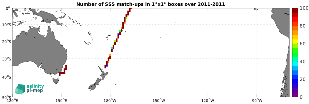
Figure 5: Number of SSS match-ups between TSG (CSIC-UTM) SSS and the SMOS SSS L3 v2 - 9-Days (BEC) SSS product for the South Pacific Ocean Pi-MEP region over 1^\circ \times 1^\circ boxes and for the full satellite product period.
