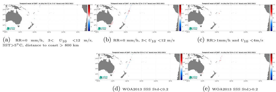
Figure 14: Temporal mean gridded over spatial boxes of size 1^\circ \times 1^\circ of \Delta\text{SSS} (SMOS SSS L3 v2 - 9-Days (BEC) - TSG (CSIC-UTM)) for 5 different subdatasets corresponding to:RR=0 mm/h, 3 < U_{10} < 12 m/s, SST>5°C, distance to coast > 800 km (a), RR=0 mm/h, 3 < U_{10} < 12 m/s (b), RR>1mm/h and U_{10} < 4 m/s (c), WOA2013 SSS Std<0.2 (d), WOA2013 SSS Std>0.2 (e).
