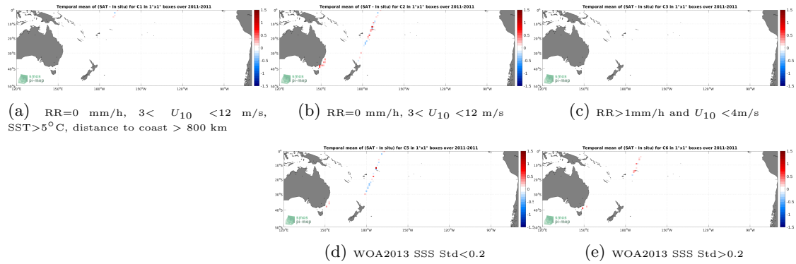
Figure 12: Temporal mean gridded over spatial boxes of size 1^\circ \times 1^\circ of \Delta SSS (SMOS SSS L3 v2 - 9-Days (BEC) - TSG (CSIC-UTM)) for 5 different subdatasets corresponding to:RR=0 mm/h, 3 < U_{10} < 12 m/s, SST >5^\circ\text{C} , distance to coast > 800 km (a), RR=0 mm/h, 3 < U_{10} < 12 m/s (b), RR >1 mm/h and U_{10} < 4 m/s (c), WOA2013 SSS Std <0.2 (d), WOA2013 SSS Std >0.2 (e).
