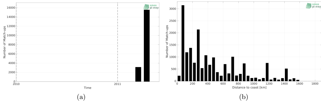
Figure 1: Number of match-ups between TSG (CSIC-UTM) and SMOS SSS L3 v2 - 9-Days (BEC) SSS as a function of time (a) and as function of the distance to coast (b) over the South Pacific Ocean Pi-MEP region and for the full satellite product period.
