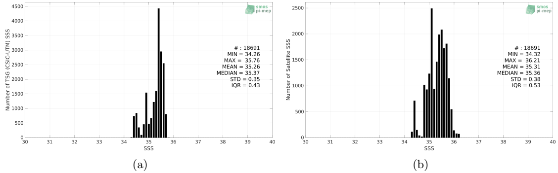
Figure 2: Histograms of SSS from TSG (CSIC-UTM) (a) and SMOS SSS L3 v2 - 9-Days (BEC) (b) considering all match-up pairs per bins of 0.1 over the South Pacific Ocean Pi-MEP region and for the full satellite product period.
