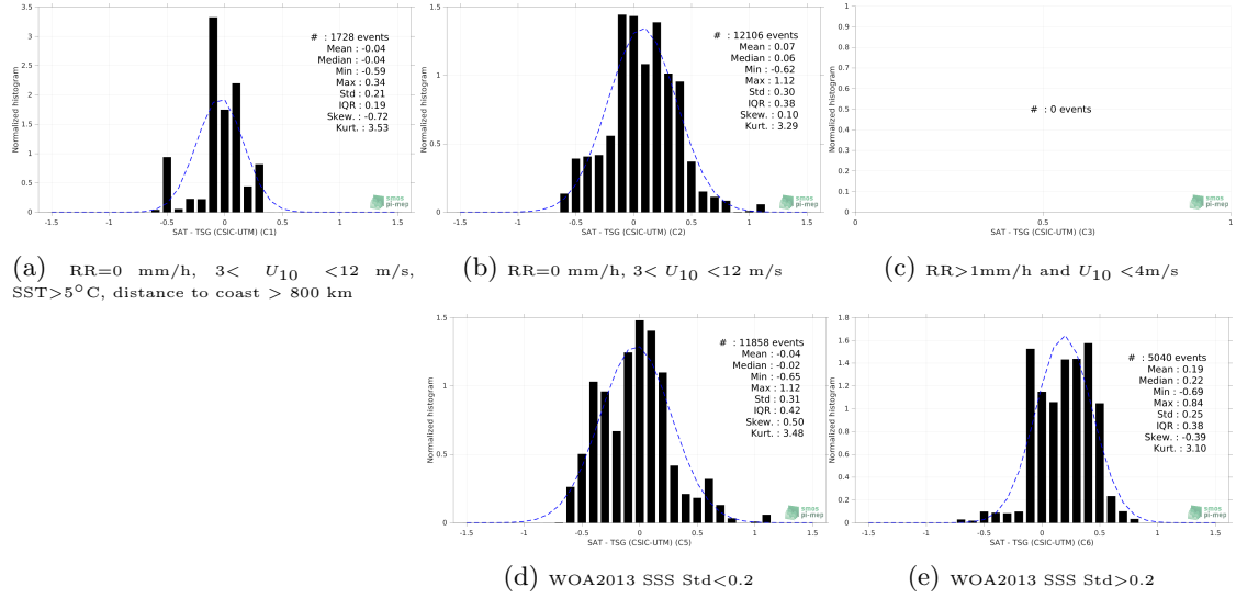
Figure 13: Normalized histogram of \Delta SSS (SMOS SSS L3 v2 - 9-Days (BEC) - TSG (CSIC-UTM)) for 5 different subdatasets corresponding to: RR=0 mm/h, 3 < U_{10} < 12 m/s, SST>5°C, distance to coast > 800 km (a), RR=0 mm/h, 3 < U_{10} < 12 m/s (b), RR>1mm/h and U_{10} < 4 m/s (c), WOA2013 SSS Std<0.2 (d), WOA2013 SSS Std>0.2 (e).
