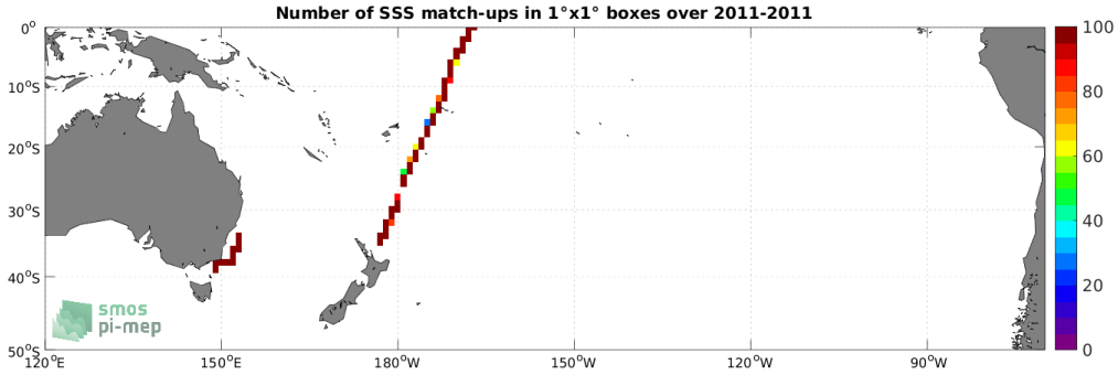
Figure 4: Number of SSS match-ups between TSG (CSIC-UTM) SSS and the SMOS SSS L3 v2 - 9-Days (BEC) SSS product for the South Pacific Ocean Pi-MEP region over 1^\circ \times 1^\circ boxes and for the full satellite product period.
