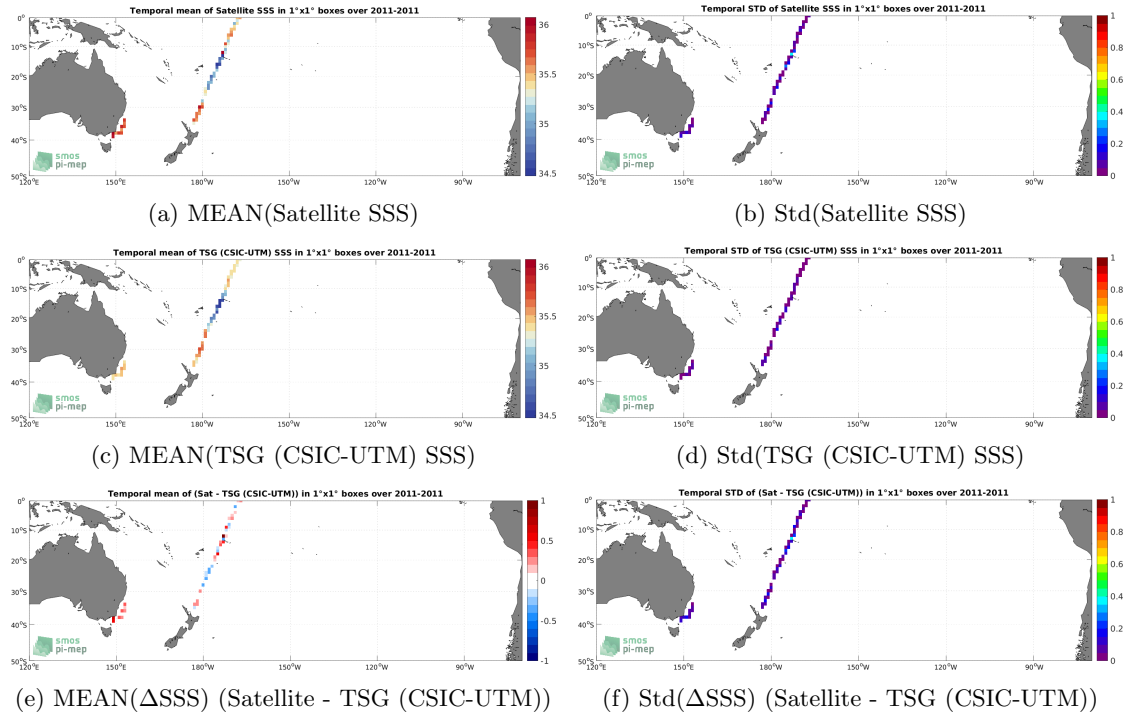
Figure 6: Temporal mean (left) and Std (right) of SSS from SMOS SSS L3 v2 - 9-Days (BEC) (top), TSG (CSIC-UTM) (middle), and of \Delta SSS (Satellite - TSG (CSIC-UTM)). Only match-up pairs are used to generate these maps.
