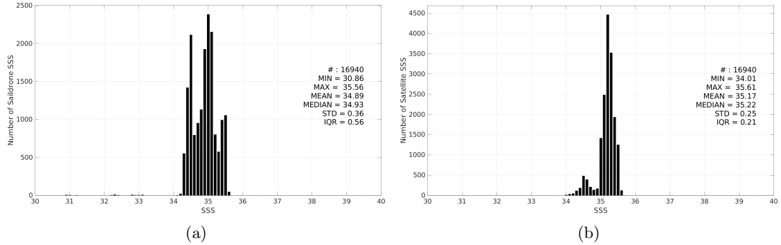
Figure 3: Histograms of SSS from Saildrone (a) and SMOS SSS L3 v2 - 9-Days (BEC) (b) considering all match-up pairs per bins of 0.1 over the South Pacific Ocean Pi-MEP region and for the full satellite product period.
