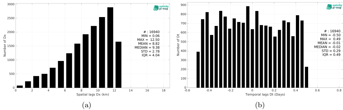
Figure 6: Histograms of the spatial (a) and temporal (b) lags between the location/time of the Sairdrone measurement and the date of the corresponding SMOS SSS L3 v2 - 9-Days (BEC) SSS pixel.
