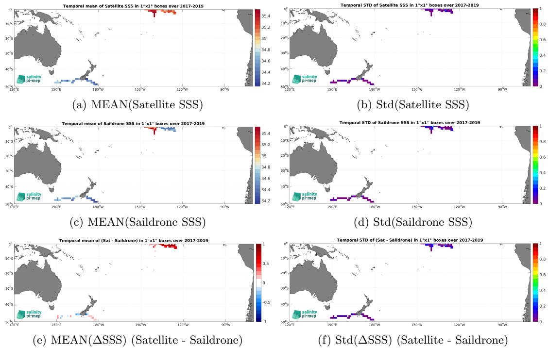
Figure 7: Temporal mean (left) and Std (right) of SSS from SMOS SSS L3 v2 - 9-Days (BEC) (top), Saildrone (middle), and of \Delta SSS (Satellite - Saildrone). Only match-up pairs are used to generate these maps.
