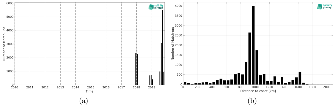
Figure 2: Number of match-ups between Saildrone and SMOS SSS L3 v2 - 9-Days (BEC) SSS as a function of time (a) and as function of the distance to coast (b) over the South Pacific Ocean Pi-MEP region and for the full satellite product period.
