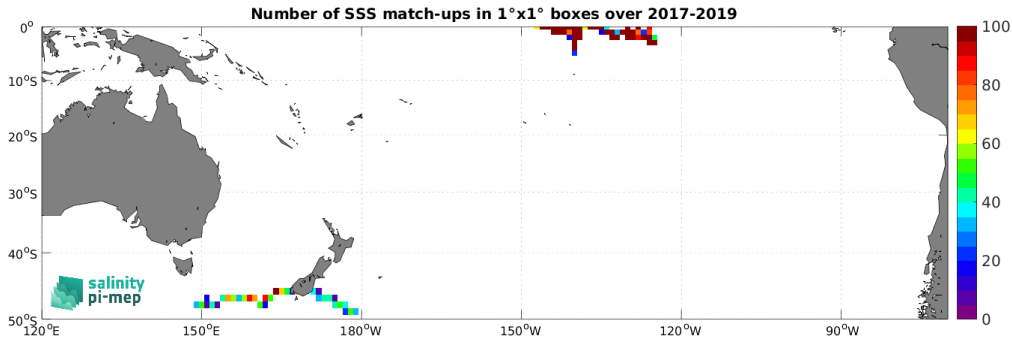
Figure 5: Number of SSS match-ups between Sairdrone SSS and the SMOS SSS L3 v2 - 9-Days (BEC) SSS product for the South Pacific Ocean Pi-MEP region over 1^\circ \times 1^\circ boxes and for the full satellite product period.
