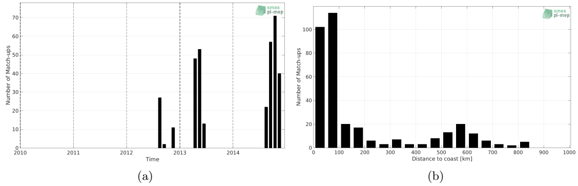
Figure 1: Number of match-ups between Sea mammals and SMOS SSS L3 v2 - 9-Days (BEC) SSS as a function of time (a) and as function of the distance to coast (b) over the South Pacific Ocean Pi-MEP region and for the full satellite product period.
