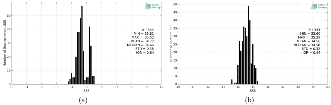
Figure 2: Histograms of SSS from Sea mammals (a) and SMOS SSS L3 v2 - 9-Days (BEC) (b) considering all match-up pairs per bins of 0.1 over the South Pacific Ocean Pi-MEP region and for the full satellite product period.
