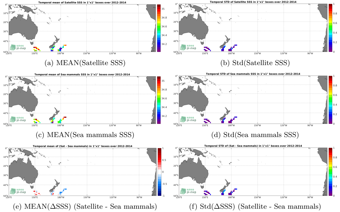
Figure 6: Temporal mean (left) and Std (right) of SSS from SMOS SSS L3 v2 - 9-Days (BEC) (top), Sea mammals (middle), and of \Delta SSS (Satellite - Sea mammals). Only match-up pairs are used to generate these maps.
