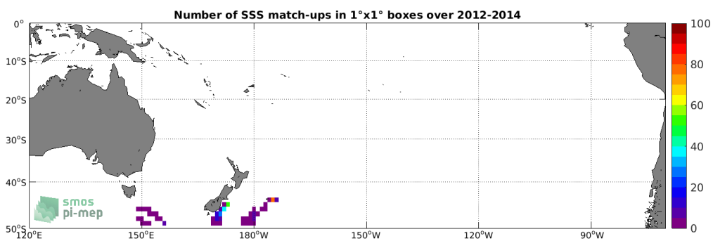
Figure 4: Number of SSS match-ups between Sea mammals SSS and the SMOS SSS L3 v2 - 9-Days (BEC) SSS product for the South Pacific Ocean Pi-MEP region over 1^\circ \times 1^\circ boxes and for the full satellite product period.
