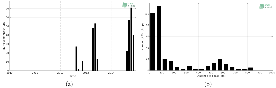
Figure 1: Number of match-ups between Sea mammals and SMOS L3 v2 - 9-Days (BEC) SSS as a function of time (a) and as function of the distance to coast (b) over the South Pacific Ocean Pi-MEP region and for the full satellite product period.
