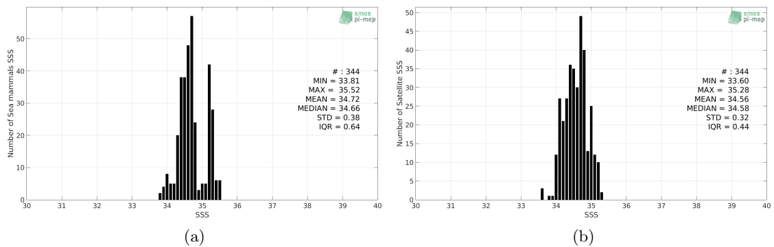
Figure 2: Histograms of SSS from Sea mammals (a) and SMOS L3 v2 - 9-Days (BEC) (b) considering all match-up pairs per bins of 0.1 over the South Pacific Ocean Pi-MEP region and for the full satellite product period.
