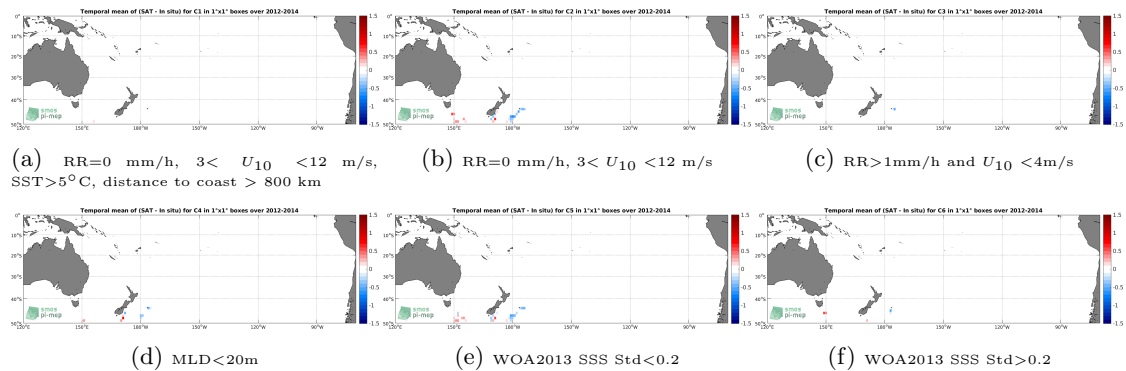
Figure 12: Temporal mean gridded over spatial boxes of size 1^{\circ}\times 1^{\circ} of \Delta\text{SSS} (SMOS L3 v2 - 9-Days (BEC) - Sea mammals) for 6 different subdatasets corresponding to: \text{RR}=0 mm/h, 3 < U_{10} < 12 m/s, SST > 5^{\circ}\text{C} , distance to coast > 800 km (a), \text{RR}=0 mm/h, 3 < U_{10} < 12 m/s (b), \text{RR} > 1\text{mm/h} and U_{10} < 4\text{m/s} (c), \text{MLD} < 20\text{m} (d), WOA2013 SSS Std < 0.2 (e), WOA2013 SSS Std > 0.2 (f).
