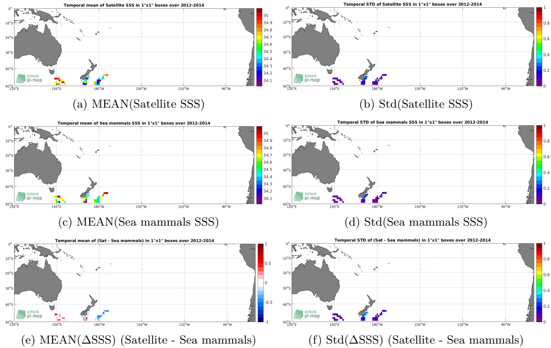
Figure 6: Temporal mean (left) and Std (right) of SSS from SMOS L3 v2 - 9-Days (BEC) (top), Sea mammals (middle), and of \Delta SSS (Satellite - Sea mammals). Only match-up pairs are used to generate these maps.
