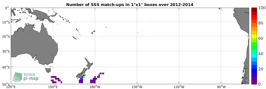
Figure 4: Number of SSS match-ups between Sea mammals SSS and the SMOS L3 v2 - 9-Days (BEC) SSS product for the South Pacific Ocean Pi-MEP region over 1^\circ \times 1^\circ boxes and for the full satellite product period.
