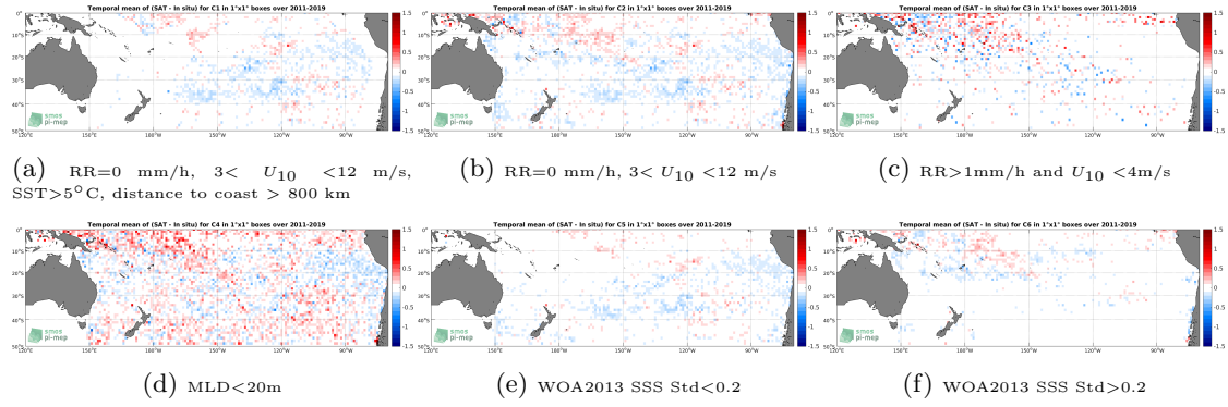
Figure 12: Temporal mean gridded over spatial boxes of size 1^\circ \times 1^\circ of \Delta SSS (SMOS SSS L3 v2 - 9-Days (BEC) - Argo) for 6 different subdatasets corresponding to: RR=0 mm/h, 3 < U_{10} < 12 m/s, SST > 5^\circ C , distance to coast > 800 km (a), RR=0 mm/h, 3 < U_{10} < 12 m/s (b), RR > 1 mm/h and U_{10} < 4 m/s (c), MLD < 20 m (d), WOA2013 SSS Std < 0.2 (e), WOA2013 SSS Std > 0.2 (f).
