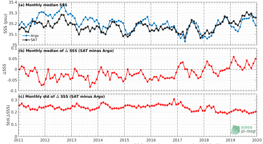
Figure 7: Time series of the monthly median SSS (top), median of \Delta\text{SSS} (Satellite - Argo) and Std of \Delta\text{SSS} (Satellite - Argo) over the South Pacific Ocean Pi-MEP region considering all match-ups collected by the Pi-MEP.
