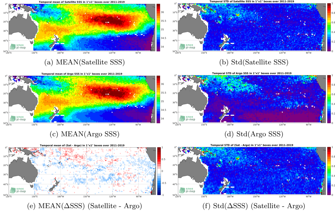
Figure 6: Temporal mean (left) and Std (right) of SSS from SMOS L3 v2 - 9-Days (BEC) (top), Argo (middle), and of \Delta SSS (Satellite - Argo). Only match-up pairs are used to generate these maps.
