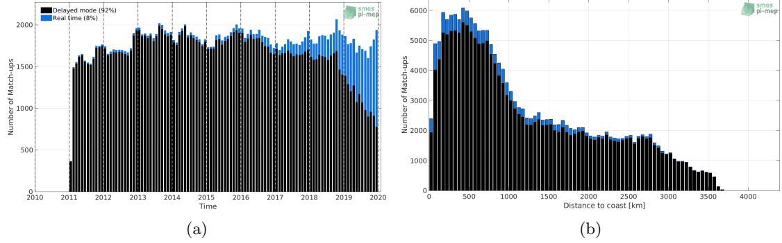
Figure 1: Number of match-ups between Argo and SMOS L3 v2 - 9-Days (BEC) SSS as a function of time (a) and as function of the distance to coast (b) over the South Pacific Ocean Pi-MEP region and for the full satellite product period.
