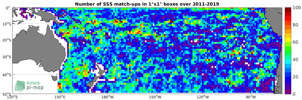
Figure 4: Number of SSS match-ups between Argo SSS and the SMOS L3 v2 - 9-Days (BEC) SSS product for the South Pacific Ocean Pi-MEP region over 1^\circ \times 1^\circ boxes and for the full satellite product period.
