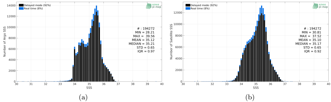
Figure 2: Histograms of SSS from Argo (a) and SMOS L3 v2 - 9-Days (BEC) (b) considering all match-up pairs per bins of 0.1 over the South Pacific Ocean Pi-MEP region and for the full satellite product period.
