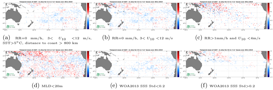
Figure 12: Temporal mean gridded over spatial boxes of size 1^\circ \times 1^\circ of \Delta SSS (SMOS L3 v2 - 9-Days (BEC) - Argo) for 6 different subdatasets corresponding to: RR=0 mm/h, 3 < U_{10} < 12 m/s, SST > 5^\circ C , distance to coast > 800 km (a), RR=0 mm/h, 3 < U_{10} < 12 m/s (b), RR > 1 mm/h and U_{10} < 4 m/s (c), MLD < 20 m (d), WOA2013 SSS Std < 0.2 (e), WOA2013 SSS Std > 0.2 (f).
