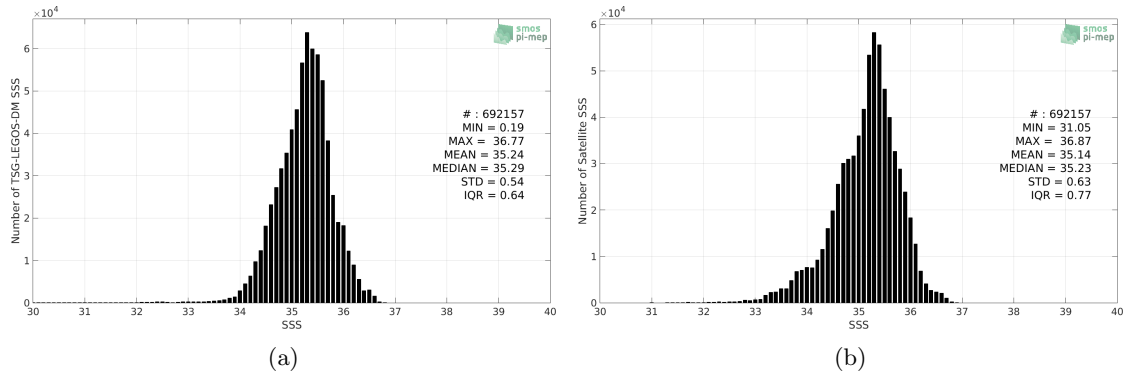
Figure 2: Histograms of SSS from TSG-LEGOS-DM (a) and SMOS-L3-BEC-OA-V1-9DAYS-0.25DEG (b) considering all match-up pairs per bins of 0.1 over the South Pacific Ocean Pi-MEP region and for the full satellite product period.
