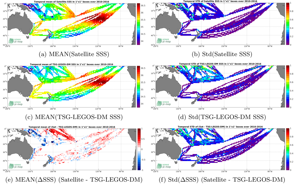
Figure 6: Temporal mean (left) and Std (right) of SSS from SMOS-L3-BEC-OA-V1-9DAYS-0.25DEG (top), TSG-LEGOS-DM (middle), and of \Delta SSS (Satellite - TSG-LEGOS-DM). Only match-up pairs are used to generate these maps.
