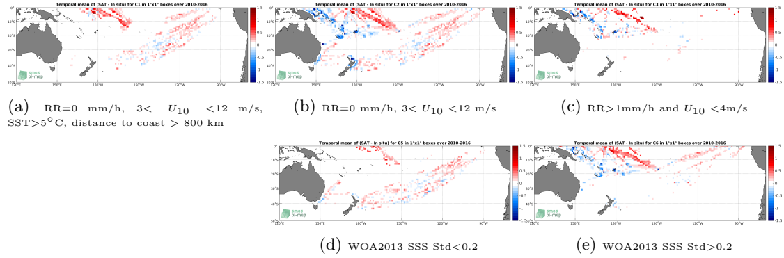
Figure 12: Temporal mean gridded over spatial boxes of size 1^\circ \times 1^\circ of \Delta SSS (SMOS-L3-BEC-OA-V1-9DAYS-0.25DEG - TSG-LEGOS-DM) for 5 different subdatasets corresponding to: RR=0 mm/h, 3 < U_{10} < 12 m/s, SST > 5^\circ C , distance to coast > 800 km (a), RR=0 mm/h, 3 < U_{10} < 12 m/s (b), RR > 1 mm/h and U_{10} < 4 m/s (c), WOA2013 SSS Std < 0.2 (d), WOA2013 SSS Std > 0.2 (e).
