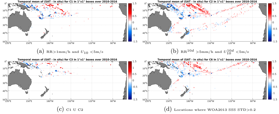
Figure 12: Temporal mean gridded over spatial boxes of size 1^\circ \times 1^\circ of \Delta SSS (SMOS-L3-BEC-OA-V1-9DAYS-0.25DEG - TSG-LEGOS-DM) for 4 different subdatasets corresponding to: RR > 1mm/h and U_{10} < 5 m/s (a), RR^{10d} > 5 mm/h and U_{10}^{10d} < 5 m/s (b), C1 U C2 (c), Locations where WOA2013 SSS STD > 0.2 (d).
