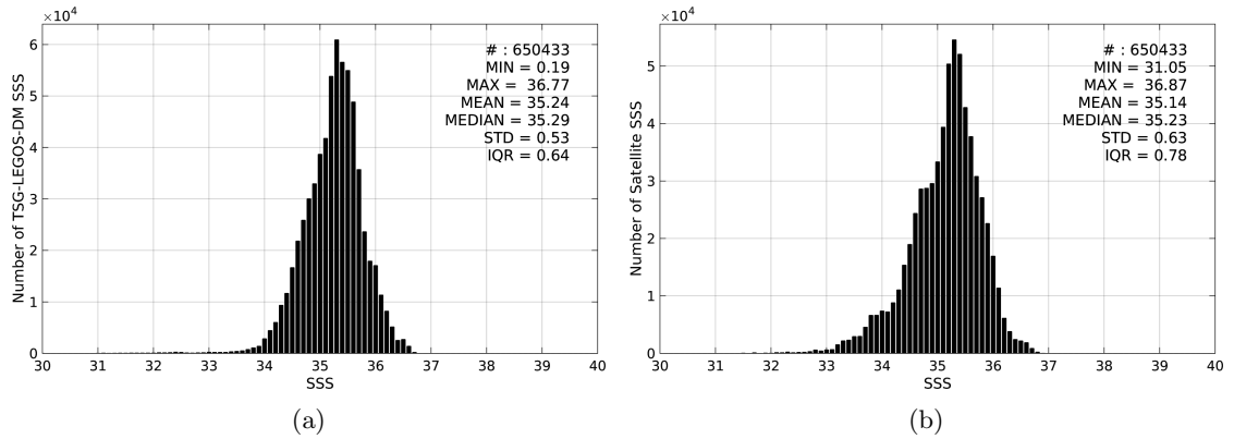
Figure 2: Histograms of SSS from TSG-LEGOS-DM (a) and SMOS-L3-BEC-OA-V1-9DAYS-0.25DEG (b) considering all match-up pairs per bins of 0.1 over the South Pacific Ocean Pi-MEP region and for the full satellite product period.
