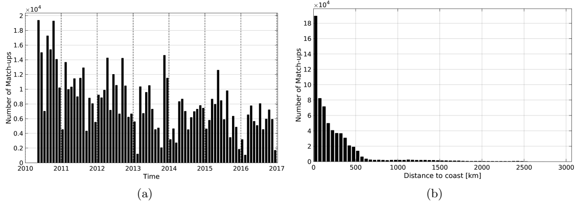
Figure 1: Number of match-ups between TSG-LEGOS-DM and SMOS-L3-BEC-OA-V1-9DAYS-0.25DEG SSS as a function of time (a) and as function of the distance to coast (b) over the South Pacific Ocean Pi-MEP region and for the full satellite product period.
