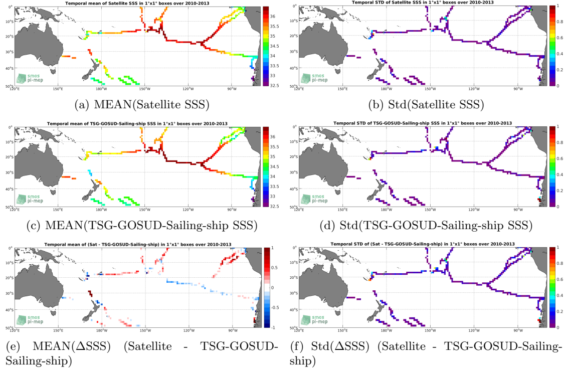
Figure 6: Temporal mean (left) and Std (right) of SSS from SMOS-L3-BEC-OA-V1-9DAYS-0.25DEG (top), TSG-GOSUD-Sailing-ship (middle), and of \Delta SSS (Satellite - TSG-GOSUD-Sailing-ship). Only match-up pairs are used to generate these maps.
