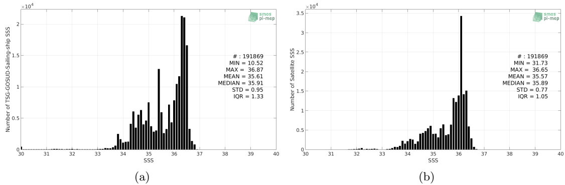
Figure 2: Histograms of SSS from TSG-GOSUD-Sailing-ship (a) and SMOS-L3-BEC-OA-V1-9DAYS-0.25DEG (b) considering all match-up pairs per bins of 0.1 over the South Pacific Ocean Pi-MEP region and for the full satellite product period.
