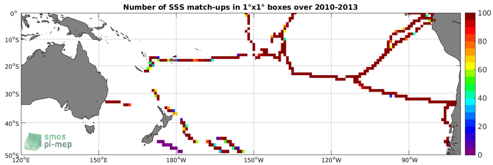
Figure 4: Number of SSS match-ups between TSG-GOSUD-Sailing-ship SSS and the SMOS-L3-BEC-OA-V1-9DAYS-0.25DEG SSS product for the South Pacific Ocean Pi-MEP region over 1^\circ \times 1^\circ boxes and for the full satellite product period.
