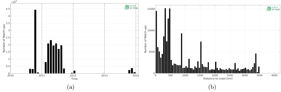
Figure 1: Number of match-ups between TSG-GOSUD-Sailing-ship and SMOS-L3-BEC-OA-V1-9DAYS-0.25DEG SSS as a function of time (a) and as function of the distance to coast (b) over the South Pacific Ocean Pi-MEP region and for the full satellite product period.
