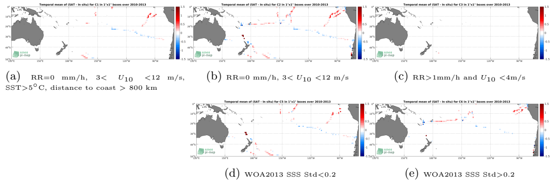
Figure 12: Temporal mean gridded over spatial boxes of size 1^\circ \times 1^\circ of \Delta SSS (SMOS-L3-BEC-OA-V1-9DAYS-0.25DEG - TSG-GOSUD-Sailing-ship) for 5 different subdatasets corresponding to: RR=0 mm/h, 3 < U_{10} < 12 m/s, SST > 5^\circ C , distance to coast > 800 km (a), RR=0 mm/h, 3 < U_{10} < 12 m/s (b), RR > 1 mm/h and U_{10} < 4 m/s (c), WOA2013 SSS Std < 0.2 (d), WOA2013 SSS Std > 0.2 (e).
