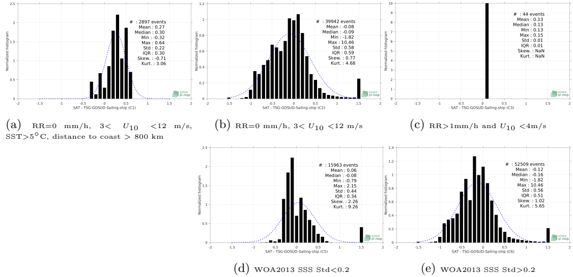
Figure 13: Normalized histogram of \Delta\text{SSS} (SMOS-L3-BEC-OA-V1-9DAYS-0.25DEG - TSG-GOSUD-Sailing-ship) for 5 different subdatasets corresponding to: RR=0 mm/h, 3 < U_{10} < 12 m/s, SST > 5^{\circ}\text{C} , distance to coast > 800 km (a), RR=0 mm/h, 3 < U_{10} < 12 m/s (b), RR > 1\text{mm/h} and U_{10} < 4\text{m/s} (c), WOA2013 SSS Std < 0.2 (d), WOA2013 SSS Std > 0.2 (e).
