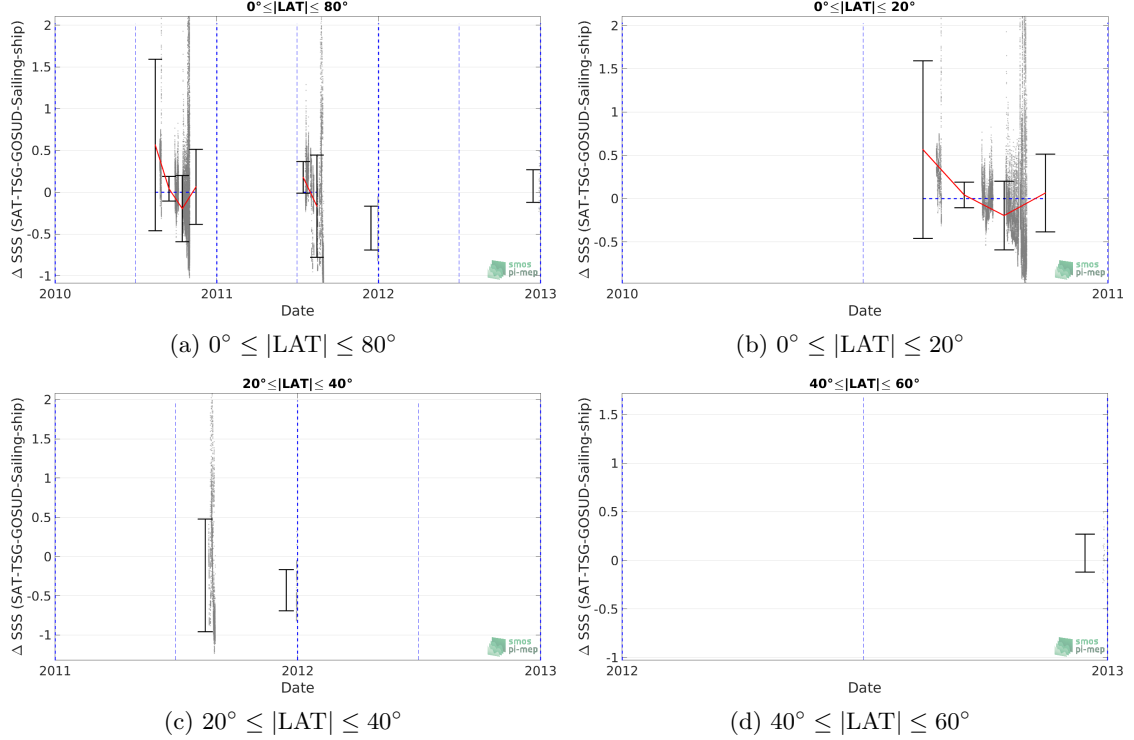
Figure 10: Monthly-averaged mean (red curves) \Delta SSS (Satellite - TSG-GOSUD-Sailing-ship) and \pm 1 STD (black vertical thick bars) as function of time for all the collected Pi-MEP match-up pairs estimated over the South Pacific Ocean Pi-MEP region and for the full satellite product period are shown for different latitude bands: (a) Latitude band 80^\circ S-80^\circ N , (b) latitude band 20^\circ S-20^\circ N , (c) Mid Latitude bands 40^\circ S-20^\circ S and 20^\circ N-40^\circ N and (d) Latitude bands 60^\circ S-40^\circ S and 40^\circ N-60^\circ N .
