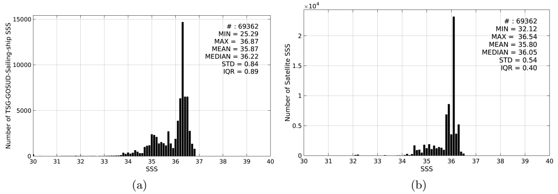
Figure 2: Histograms of SSS from TSG-GOSUD-Sailing-ship (a) and SMOS-L3-BEC-OA-V1-9DAYS-0.25DEG (b) considering all match-up pairs per bins of 0.1 over the South Pacific Ocean Pi-MEP region and for the full satellite product period.
