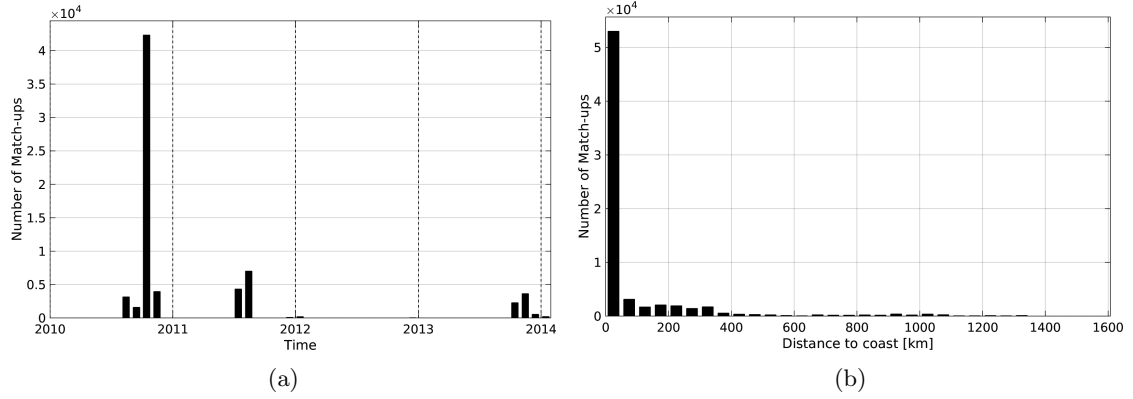
Figure 1: Number of match-ups between TSG-GOSUD-Sailing-ship and SMOS-L3-BEC-OA-V1-9DAYS-0.25DEG SSS as a function of time (a) and as function of the distance to coast (b) over the South Pacific Ocean Pi-MEP region and for the full satellite product period.
