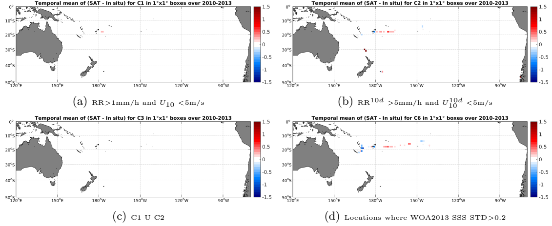
Figure 12: Temporal mean gridded over spatial boxes of size 1^\circ \times 1^\circ of \Delta SSS (SMOS-L3-BEC-OA-V1-9DAYS-0.25DEG - TSG-GOSUD-Sailing-ship) for 4 different subdatasets corresponding to: RR > 1 mm/h and U_{10} < 5 m/s (a), RR^{10d} > 5 mm/h and U_{10}^{10d} < 5 m/s (b), C1 U C2 (c), Locations where WOA2013 SSS STD > 0.2 (d).
