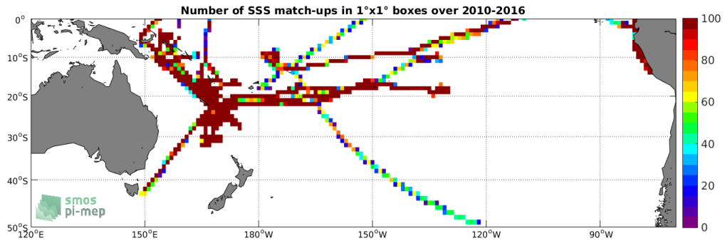
Figure 4: Number of SSS match-ups between TSG-GOSUD-Research-vessel SSS and the SMOS-L3-BEC-OA-V1-9DAYS-0.25DEG SSS product for the South Pacific Ocean Pi-MEP region over 1°x1° boxes and for the full satellite product period.
