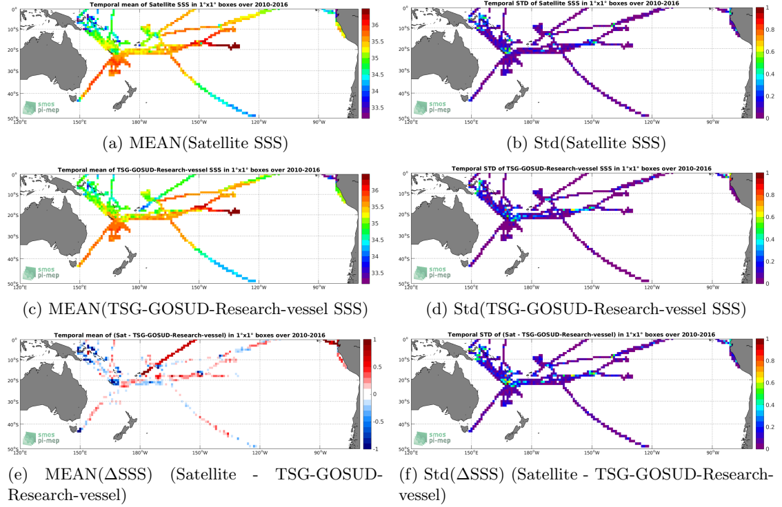
Figure 6: Temporal mean (left) and Std (right) of SSS from SMOS-L3-BEC-OA-V1-9DAYS-0.25DEG (top), TSG-GOSUD-Research-vessel (middle), and of \Delta SSS (Satellite - TSG-GOSUD-Research-vessel). Only match-up pairs are used to generate these maps.
