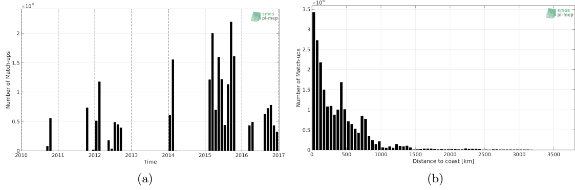
Figure 1: Number of match-ups between TSG-GOSUD-Research-vessel and SMOS-L3-BEC-OA-V1-9DAYS-0.25DEG SSS as a function of time (a) and as function of the distance to coast (b) over the South Pacific Ocean Pi-MEP region and for the full satellite product period.
