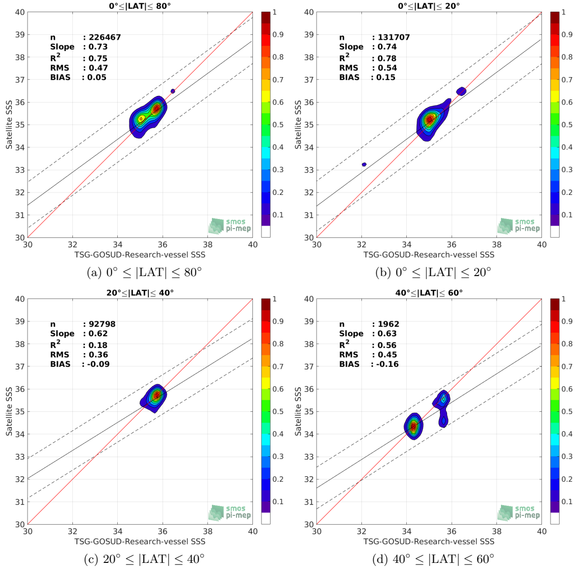
Figure 9: Contour maps of the concentration of SMOS-L3-BEC-OA-V1-9DAYS-0.25DEG SSS (y-axis) versus TSG-GOSUD-Research-vessel SSS (x-axis) at match-up pairs for different latitude bands. For each plot, the red line shows x=y . The black thin and dashed lines indicate a linear fit through the data cloud and the \pm 95\% confidence levels, respectively. The number match-up pairs n , the slope and R^2 coefficient of the linear fit, the root mean square (RMS) and the mean bias between satellite and in situ data are indicated for each latitude band in each plots.
