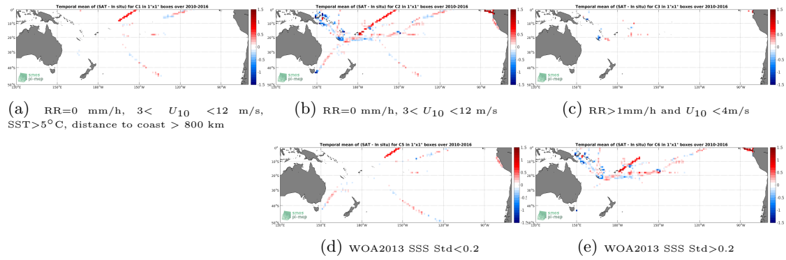
Figure 12: Temporal mean gridded over spatial boxes of size 1^\circ \times 1^\circ of \Delta SSS (SMOS-L3-BEC-OA-V1-9DAYS-0.25DEG - TSG-GOSUD-Research-vessel) for 5 different subdatasets corresponding to: RR=0 mm/h, 3 < U_{10} < 12 m/s, SST > 5^\circ C , distance to coast > 800 km (a), RR=0 mm/h, 3 < U_{10} < 12 m/s (b), RR > 1 mm/h and U_{10} < 4 m/s (c), WOA2013 SSS Std < 0.2 (d), WOA2013 SSS Std > 0.2 (e).
