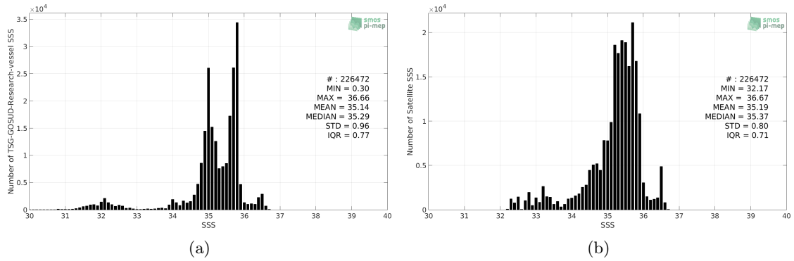
Figure 2: Histograms of SSS from TSG-GOSUD-Research-vessel (a) and SMOS-L3-BEC-OA-V1-9DAYS-0.25DEG (b) considering all match-up pairs per bins of 0.1 over the South Pacific Ocean Pi-MEP region and for the full satellite product period.
