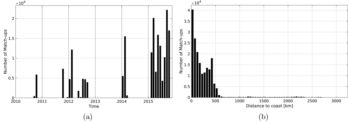
Figure 1: Number of match-ups between TSG-GOSUD-Research-vessel and SMOS-L3-BEC-OA-V1-9DAYS-0.25DEG SSS as a function of time (a) and as function of the distance to coast (b) over the South Pacific Ocean Pi-MEP region and for the full satellite product period.
