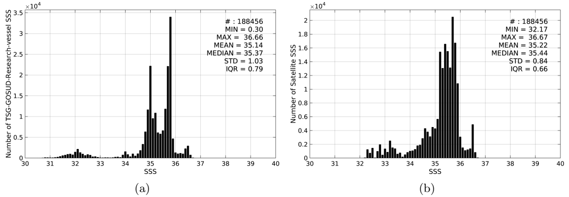
Figure 2: Histograms of SSS from TSG-GOSUD-Research-vessel (a) and SMOS-L3-BEC-OA-V1-9DAYS-0.25DEG (b) considering all match-up pairs per bins of 0.1 over the South Pacific Ocean Pi-MEP region and for the full satellite product period.
