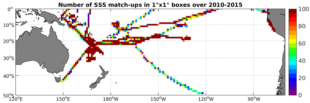
Figure 4: Number of SSS match-ups between TSG-GOSUD-Research-vessel SSS and the SMOS-L3-BEC-OA-V1-9DAYS-0.25DEG SSS product for the South Pacific Ocean Pi-MEP region over 1^\circ \times 1^\circ boxes and for the full satellite product period.
