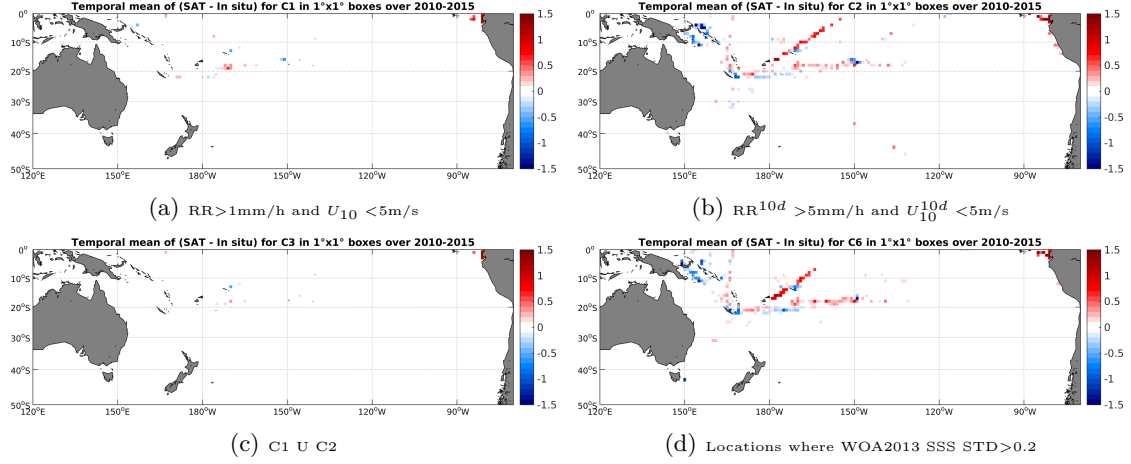
Figure 12: Temporal mean gridded over spatial boxes of size 1^\circ \times 1^\circ of \Delta SSS (SMOS-L3-BEC-OA-V1-9DAYS-0.25DEG - TSG-GOSUD-Research-vessel) for 4 different subdatasets corresponding to: RR > 1mm/h and U_{10} < 5 m/s (a), RR^{10d} > 5 mm/h and U_{10}^{10d} < 5 m/s (b), C1 U C2 (c), Locations where WOA2013 SSS STD > 0.2 (d).
