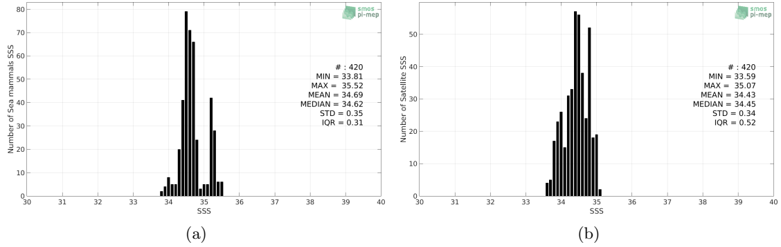
Figure 2: Histograms of SSS from Sea mammals (a) and SMOS-L3-BEC-OA-V1-9DAYS-0.25DEG (b) considering all match-up pairs per bins of 0.1 over the South Pacific Ocean Pi-MEP region and for the full satellite product period.
