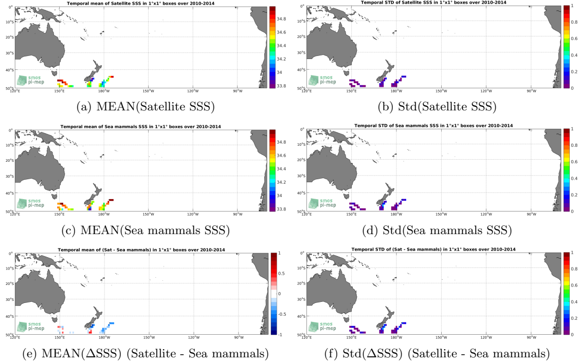
Figure 6: Temporal mean (left) and Std (right) of SSS from SMOS-L3-BEC-OA-V1-9DAYS-0.25DEG (top), Sea mammals (middle), and of \Delta SSS (Satellite - Sea mammals). Only match-up pairs are used to generate these maps.
