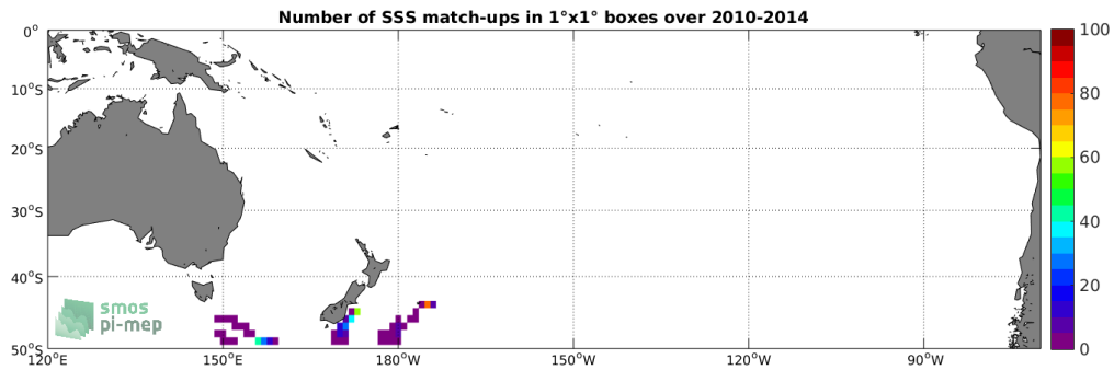
Figure 4: Number of SSS match-ups between Sea mammals SSS and the SMOS-L3-BEC-OA-V1-9DAYS-0.25DEG SSS product for the South Pacific Ocean Pi-MEP region over 1^\circ \times 1^\circ boxes and for the full satellite product period.
