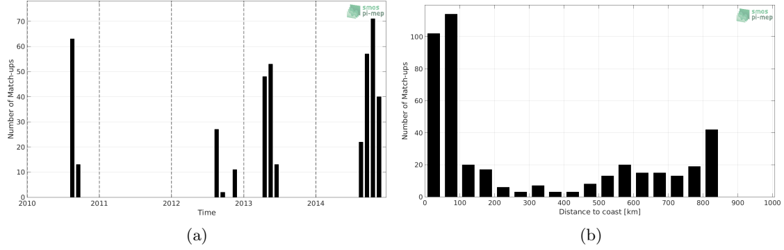
Figure 1: Number of match-ups between Sea mammals and SMOS-L3-BEC-OA-V1-9DAYS-0.25DEG SSS as a function of time (a) and as function of the distance to coast (b) over the South Pacific Ocean Pi-MEP region and for the full satellite product period.
