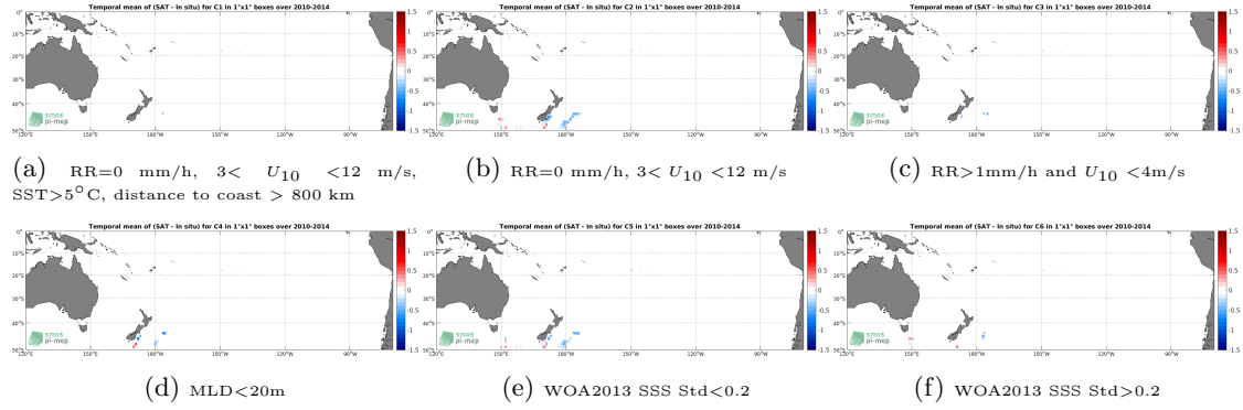
Figure 12: Temporal mean gridded over spatial boxes of size 1^\circ \times 1^\circ of \Delta SSS (SMOS-L3-BEC-OA-V1-9DAYS-0.25DEG - Sea mammals) for 6 different subdatasets corresponding to: RR=0 mm/h, 3 < U_{10} < 12 m/s, SST > 5^\circ C , distance to coast > 800 km (a), RR=0 mm/h, 3 < U_{10} < 12 m/s (b), RR > 1 mm/h and U_{10} < 4 m/s (c), MLD < 20 m (d), WOA2013 SSS Std < 0.2 (e), WOA2013 SSS Std > 0.2 (f).
