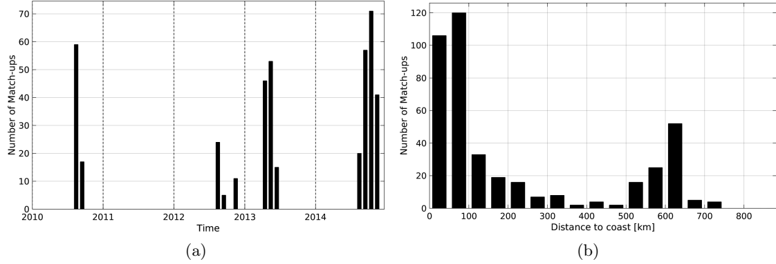
Figure 1: Number of match-ups between Sea mammals and SMOS-L3-BEC-OA-V1-9DAYS-0.25DEG SSS as a function of time (a) and as function of the distance to coast (b) over the South Pacific Ocean Pi-MEP region and for the full satellite product period.
