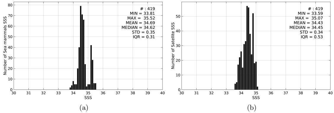
Figure 2: Histograms of SSS from Sea mammals (a) and SMOS-L3-BEC-OA-V1-9DAYS-0.25DEG (b) considering all match-up pairs per bins of 0.1 over the South Pacific Ocean Pi-MEP region and for the full satellite product period.
