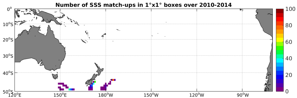
Figure 4: Number of SSS match-ups between Sea mammals SSS and the SMOS-L3-BEC-OA-V1-9DAYS-0.25DEG SSS product for the South Pacific Ocean Pi-MEP region over 1°x1° boxes and for the full satellite product period.
