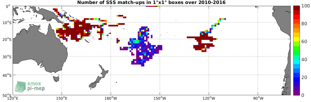
Figure 3: Number of SSS match-ups between Surface drifters SSS and the SMOS-L3-BEC-OA-V1-9DAYS-0.25DEG SSS product for the South Pacific Ocean Pi-MEP region over 1^\circ \times 1^\circ boxes and for the full satellite product period.
