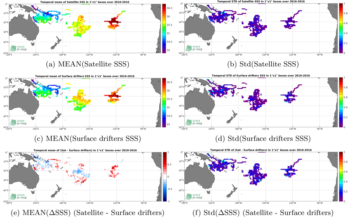
Figure 5: Temporal mean (left) and Std (right) of SSS from SMOS-L3-BEC-OA-V1-9DAYS-0.25DEG (top), Surface drifters (middle), and of \Delta SSS (Satellite - Surface drifters). Only match-up pairs are used to generate these maps.
