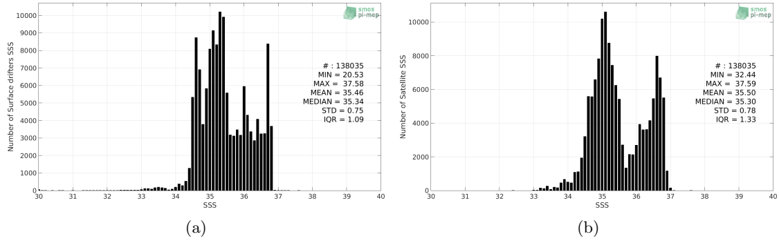
Figure 2: Histograms of SSS from Surface drifters (a) and SMOS-L3-BEC-OA-V1-9DAYS-0.25DEG (b) considering all match-up pairs per bins of 0.1 over the South Pacific Ocean Pi-MEP region and for the full satellite product period.
