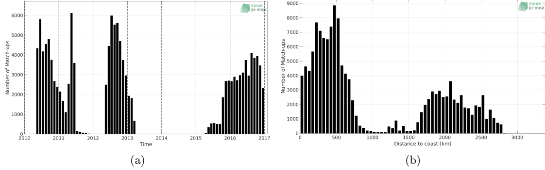
Figure 1: Number of match-ups between Surface drifters and SMOS-L3-BEC-OA-V1-9DAYS-0.25DEG SSS as a function of time (a) and as function of the distance to coast (b) over the South Pacific Ocean Pi-MEP region and for the full satellite product period.
