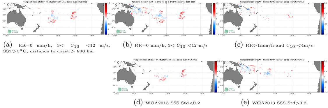
Figure 11: Temporal mean gridded over spatial boxes of size 1^\circ \times 1^\circ of \Delta SSS (SMOS-L3-BEC-OA-V1-9DAYS-0.25DEG - Surface drifters) for 5 different subdatasets corresponding to: RR=0 mm/h, 3 < U_{10} < 12 m/s, SST > 5^\circ\text{C} , distance to coast > 800 km (a), RR=0 mm/h, 3 < U_{10} < 12 m/s (b), RR > 1 mm/h and U_{10} < 4 m/s (c), WOA2013 SSS Std < 0.2 (d), WOA2013 SSS Std > 0.2 (e).
