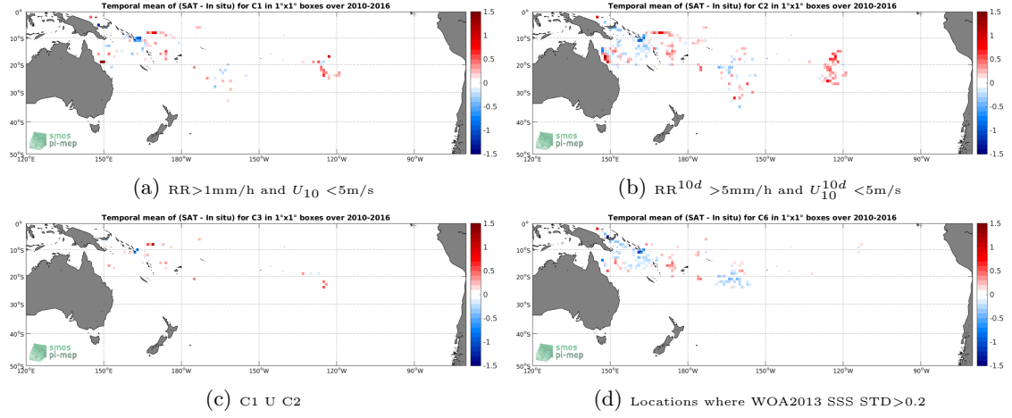
Figure 11: Temporal mean gridded over spatial boxes of size 1^\circ \times 1^\circ of \Delta SSS (SMOS-L3-BEC-OA-V1-9DAYS-0.25DEG - Surface drifters) for 4 different subdatasets corresponding to: RR > 1\text{mm/h} and U_{10} < 5\text{m/s} (a), RR^{10d} > 5\text{mm/h} and U_{10}^{10d} < 5\text{m/s} (b), C1 U C2 (c), Locations where WOA2013 SSS STD > 0.2 (d).
