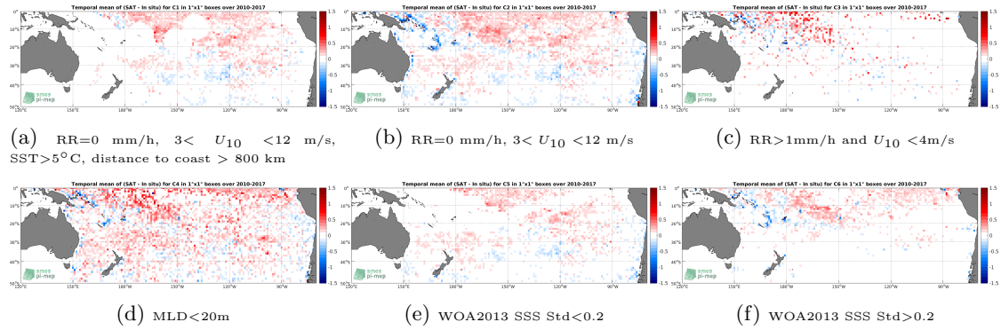
Figure 12: Temporal mean gridded over spatial boxes of size 1^\circ \times 1^\circ of \Delta SSS (SMOS-L3-BEC-OA-V1-9DAYS-0.25DEG - Argo) for 6 different subdatasets corresponding to: RR=0 mm/h, 3 < U_{10} < 12 m/s, SST > 5^\circ C , distance to coast > 800 km (a), RR=0 mm/h, 3 < U_{10} < 12 m/s (b), RR > 1 mm/h and U_{10} < 4 m/s (c), MLD < 20 m (d), WOA2013 SSS Std < 0.2 (e), WOA2013 SSS Std > 0.2 (f).
