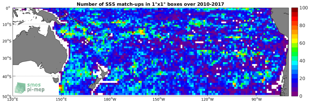
Figure 4: Number of SSS match-ups between Argo SSS and the SMOS-L3-BEC-OA-V1-9DAYS-0.25DEG SSS product for the South Pacific Ocean Pi-MEP region over 1^\circ \times 1^\circ boxes and for the full satellite product period.
