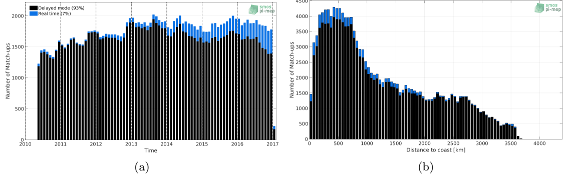
Figure 1: Number of match-ups between Argo and SMOS-L3-BEC-OA-V1-9DAYS-0.25DEG SSS as a function of time (a) and as function of the distance to coast (b) over the South Pacific Ocean Pi-MEP region and for the full satellite product period.
