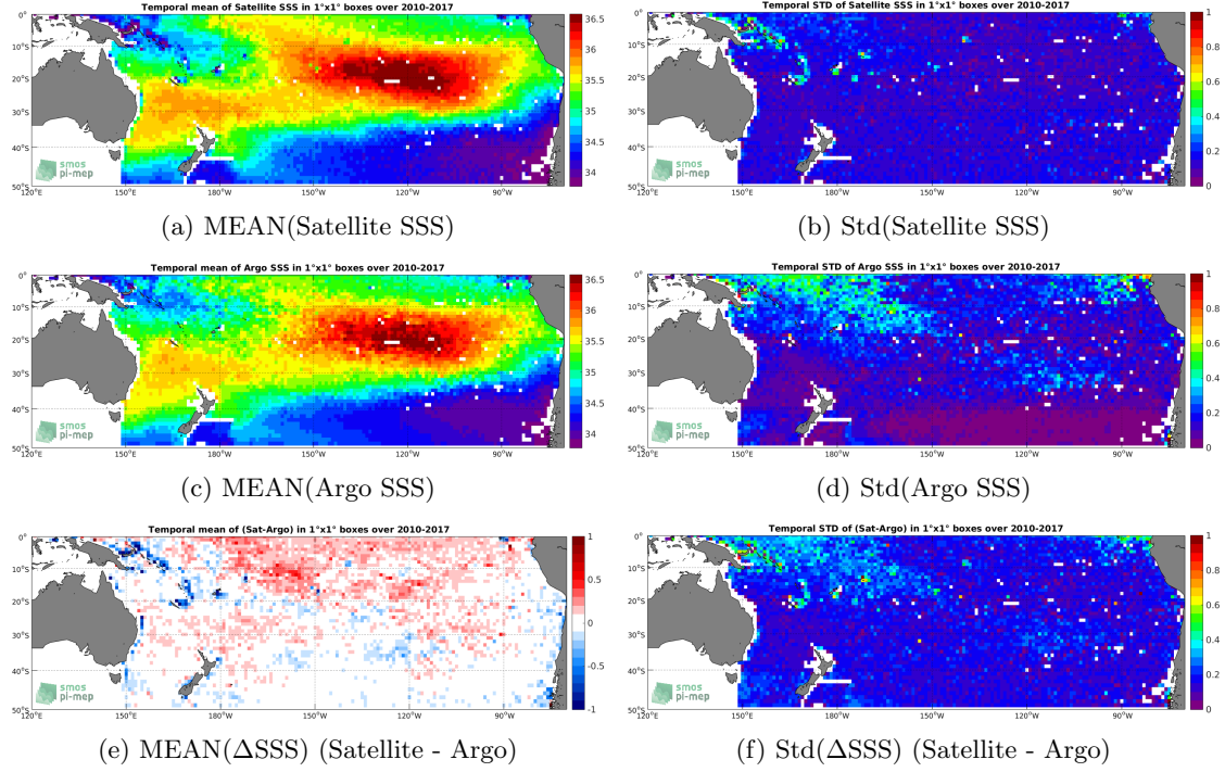
Figure 6: Temporal mean (left) and Std (right) of SSS from SMOS-L3-BEC-OA-V1-9DAYS-0.25DEG (top), Argo (middle), and of \Delta SSS (Satellite - Argo). Only match-up pairs are used to generate these maps.
