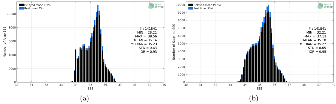
Figure 2: Histograms of SSS from Argo (a) and SMOS-L3-BEC-OA-V1-9DAYS-0.25DEG (b) considering all match-up pairs per bins of 0.1 over the South Pacific Ocean Pi-MEP region and for the full satellite product period.
