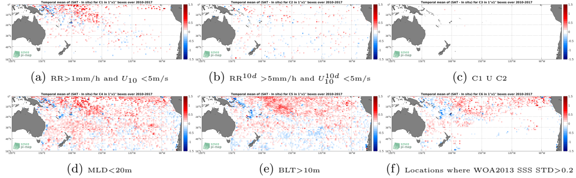
Figure 12: Temporal mean gridded over spatial boxes of size 1^\circ \times 1^\circ of \Delta\text{SSS} (SMOS-L3-BEC-OA-V1-9DAYS-0.25DEG - Argo) for 6 different subdatasets corresponding to: \text{RR}>1\text{mm/h} and U_{10}<5\text{m/s} (a), \text{RR}^{10d}>5\text{mm/h} and U_{10}^{10d}<5\text{m/s} (b), C1 U C2 (c), \text{MLD}<20\text{m} (d), \text{BLT}>10\text{m} (e), Locations where WOA2013 SSS STD >0.2 (f).
