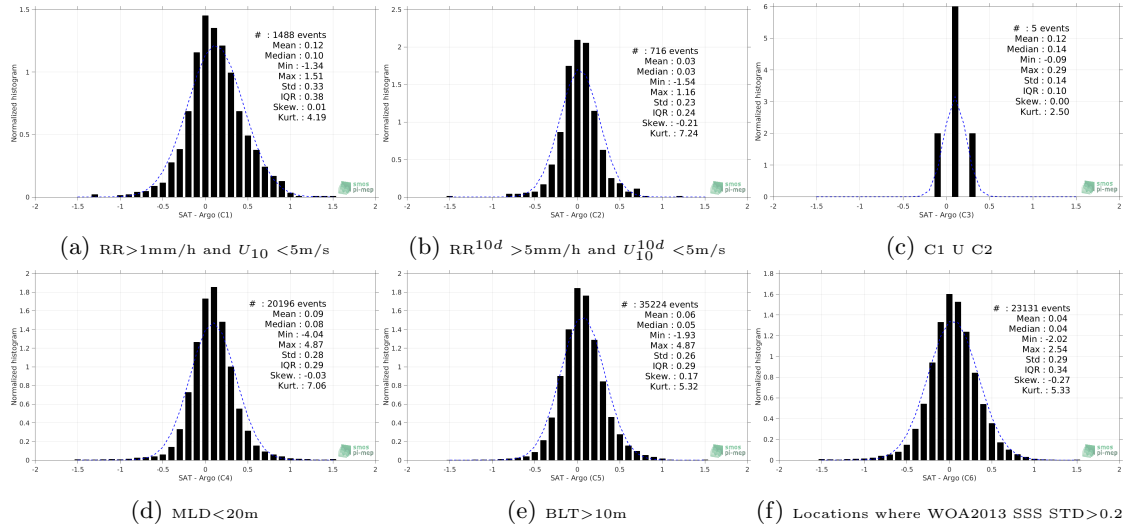
Figure 13: Normalized histogram of \Delta\text{SSS} (SMOS-L3-BEC-OA-V1-9DAYS-0.25DEG - Argo) for 6 different subdatasets corresponding to: \text{RR}>1\text{mm/h} and U_{10}<5\text{m/s} (a), \text{RR}^{10d}>5\text{mm/h} and U_{10}^{10d}<5\text{m/s} (b), C1 U C2 (c), \text{MLD}<20\text{m} (d), \text{BLT}>10\text{m} (e), Locations where WOA2013 SSS STD >0.2 (f).
