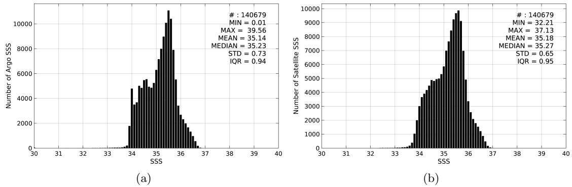
Figure 2: Histograms of SSS from Argo (a) and SMOS-L3-BEC-OA-V1-9DAYS-0.25DEG (b) considering all match-up pairs per bins of 0.1 over the South Pacific Ocean Pi-MEP region and for the full satellite product period.
