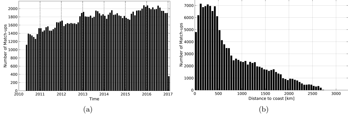
Figure 1: Number of match-ups between Argo and SMOS-L3-BEC-OA-V1-9DAYS-0.25DEG SSS as a function of time (a) and as function of the distance to coast (b) over the South Pacific Ocean Pi-MEP region and for the full satellite product period.
