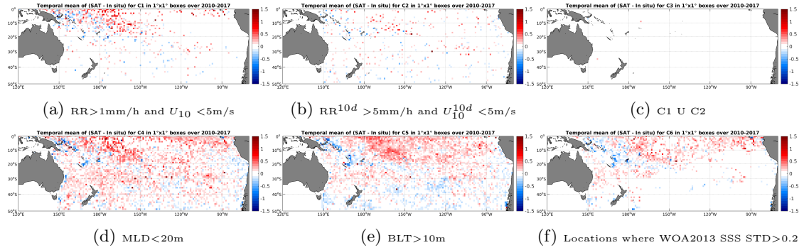
Figure 12: Temporal mean gridded over spatial boxes of size 1^\circ \times 1^\circ of \Delta SSS (SMOS-L3-BEC-OA-V1-9DAYS-0.25DEG - Argo) for 6 different subdatasets corresponding to: RR > 1\text{mm/h} and U_{10} < 5\text{m/s} (a), RR^{10d} > 5\text{mm/h} and U_{10}^{10d} < 5\text{m/s} (b), C1 U C2 (c), MLD < 20\text{m} (d), BLT > 10\text{m} (e), Locations where WOA2013 SSS STD > 0.2 (f).
