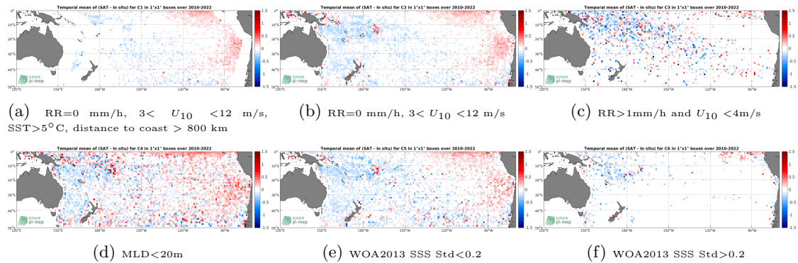
Figure 12: Temporal mean gridded over spatial boxes of size 1^\circ \times 1^\circ of \Delta SSS (SMOS SSS L2-AVERAGED v700 (ESA) - Argo) for 6 different subdatasets corresponding to:RR=0 mm/h, 3 < U_{10} < 12 m/s, SST >5^\circ\text{C} , distance to coast > 800 km (a), RR=0 mm/h, 3 < U_{10} < 12 m/s (b), RR >1 mm/h and U_{10} < 4 m/s (c),MLD <20 m (d),WOA2013 SSS Std <0.2 (e),WOA2013 SSS Std >0.2 (f).
