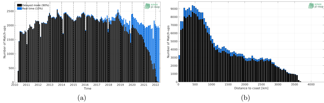
Figure 1: Number of match-ups between Argo and SMOS SSS L2-AVERAGED v700 (ESA) SSS as a function of time (a) and as function of the distance to coast (b) over the South Pacific Ocean Pi-MEP region and for the full satellite product period.
