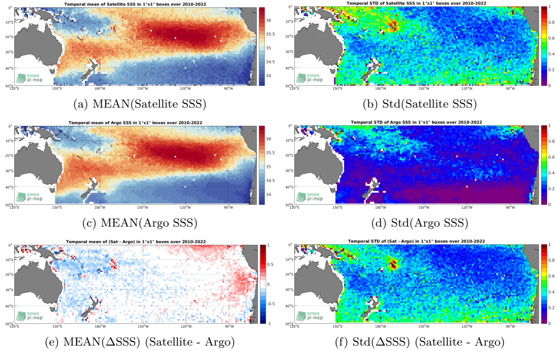
Figure 6: Temporal mean (left) and Std (right) of SSS from SMOS SSS L2-AVERAGED v700 (ESA) (top), Argo (middle), and of \Delta SSS (Satellite - Argo). Only match-up pairs are used to generate these maps.
