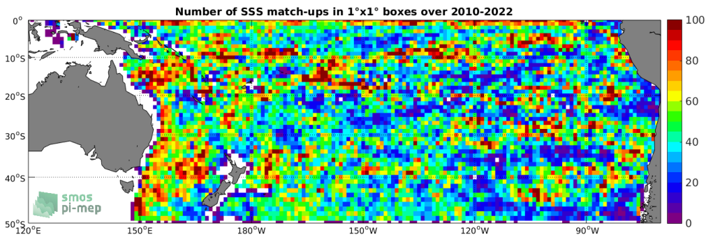
Figure 4: Number of SSS match-ups between Argo SSS and the SMOS SSS L2-AVERAGED v700 (ESA) SSS product for the South Pacific Ocean Pi-MEP region over 1^\circ \times 1^\circ boxes and for the full satellite product period.
