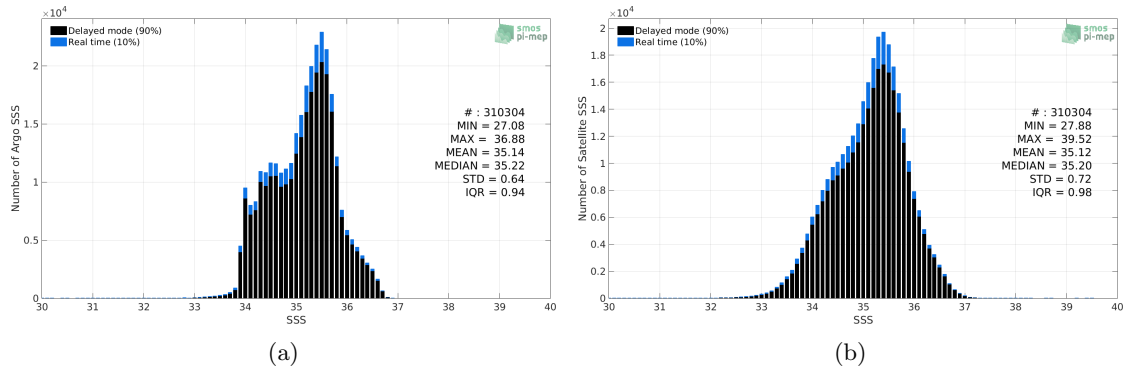
Figure 2: Histograms of SSS from Argo (a) and SMOS SSS L2-AVERAGED v700 (ESA) (b) considering all match-up pairs per bins of 0.1 over the South Pacific Ocean Pi-MEP region and for the full satellite product period.
