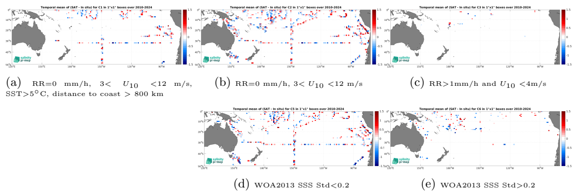
Figure 14: Temporal mean gridded over spatial boxes of size 1^\circ \times 1^\circ of \Delta\text{SSS} (SMOS SSS L2 v700 (ESA) - TSG (SAMOS)) for 5 different subdatasets corresponding to:RR=0 mm/h, 3 < U_{10} < 12 m/s, SST >5^\circ\text{C} , distance to coast > 800 km (a), RR=0 mm/h, 3 < U_{10} < 12 m/s (b), RR >1 mm/h and U_{10} < 4 m/s (c), WOA2013 SSS Std <0.2 (d), WOA2013 SSS Std >0.2 (e).
