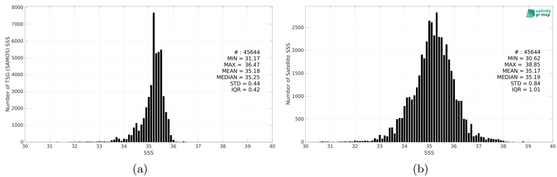
Figure 2: Histograms of SSS from TSG (SAMOS) (a) and SMOS SSS L2 v700 (ESA) (b) considering all match-up pairs per bins of 0.1 over the South Pacific Ocean Pi-MEP region and for the full satellite product period.
