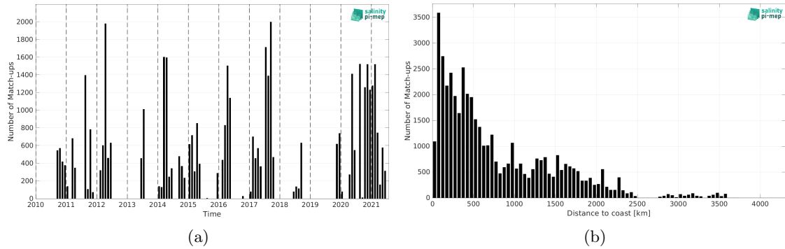
Figure 1: Number of match-ups between TSG (SAMOS) and SMOS SSS L2 v700 (ESA) SSS as a function of time (a) and as function of the distance to coast (b) over the South Pacific Ocean Pi-MEP region and for the full satellite product period.
