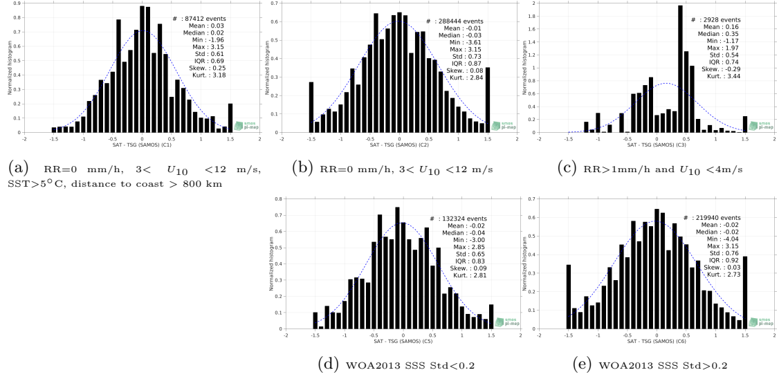
Figure 13: Normalized histogram of \Delta\text{SSS} (SMOS SSS L2 v700 (ESA) - TSG (SAMOS)) for 5 different subdatasets corresponding to: RR=0 mm/h, 3 < U_{10} < 12 m/s, SST>5°C, distance to coast > 800 km (a), RR=0 mm/h, 3 < U_{10} < 12 m/s (b), RR>1mm/h and U_{10} < 4 m/s (c), WOA2013 SSS Std<0.2 (d), WOA2013 SSS Std>0.2 (e).
