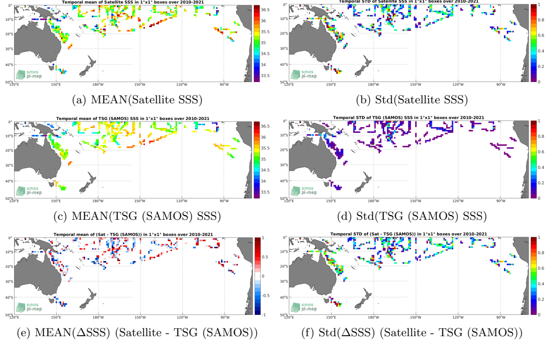
Figure 6: Temporal mean (left) and Std (right) of SSS from SMOS SSS L2 v700 (ESA) (top), TSG (SAMOS) (middle), and of \Delta\text{SSS} (Satellite - TSG (SAMOS)). Only match-up pairs are used to generate these maps.
