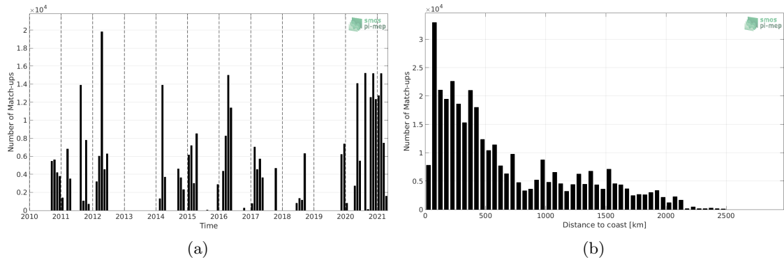
Figure 1: Number of match-ups between TSG (SAMOS) and SMOS SSS L2 v700 (ESA) SSS as a function of time (a) and as function of the distance to coast (b) over the South Pacific Ocean Pi-MEP region and for the full satellite product period.
