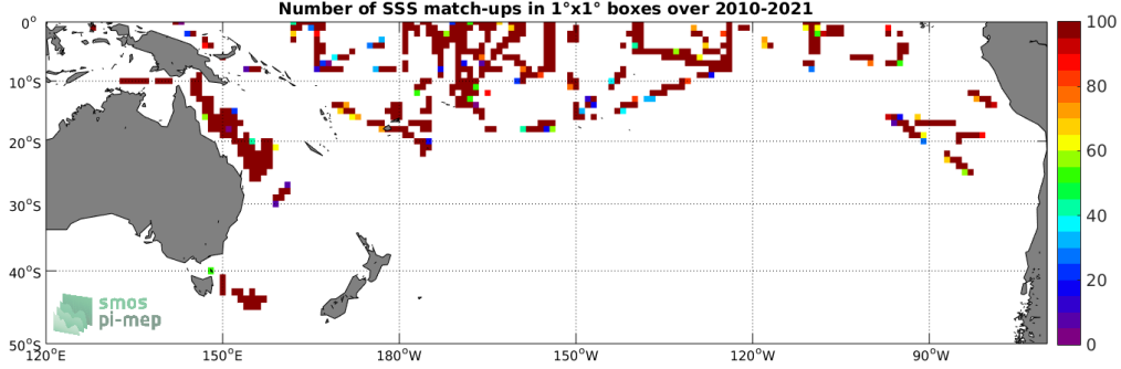
Figure 4: Number of SSS match-ups between TSG (SAMOS) SSS and the SMOS SSS L2 v700 (ESA) SSS product for the South Pacific Ocean Pi-MEP region over 1^\circ \times 1^\circ boxes and for the full satellite product period.
