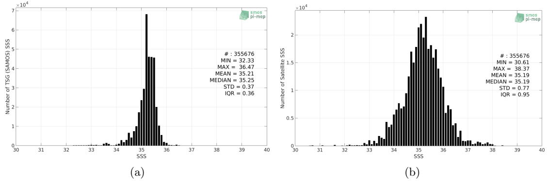
Figure 2: Histograms of SSS from TSG (SAMOS) (a) and SMOS SSS L2 v700 (ESA) (b) considering all match-up pairs per bins of 0.1 over the South Pacific Ocean Pi-MEP region and for the full satellite product period.
