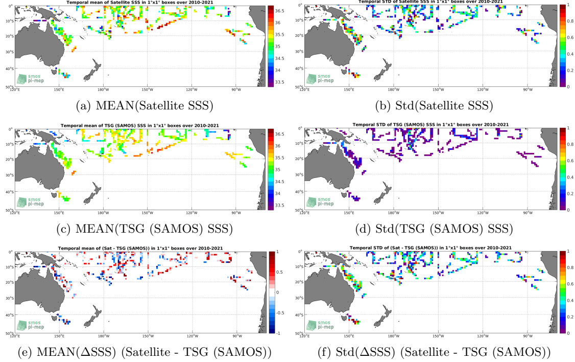
Figure 6: Temporal mean (left) and Std (right) of SSS from SMOS SSS L2 v700 (ESA) (top), TSG (SAMOS) (middle), and of \Delta SSS (Satellite - TSG (SAMOS)). Only match-up pairs are used to generate these maps.
