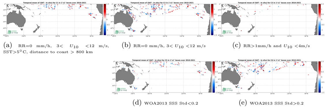
Figure 12: Temporal mean gridded over spatial boxes of size 1^\circ \times 1^\circ of \Delta SSS (SMOS SSS L2 v700 (ESA) - TSG (SAMOS)) for 5 different subdatasets corresponding to: RR=0 mm/h, 3 < U_{10} < 12 m/s, SST >5^\circ\text{C} , distance to coast > 800 km (a), RR=0 mm/h, 3 < U_{10} < 12 m/s (b), RR>1\text{mm/h} and U_{10} < 4\text{m/s} (c), WOA2013 SSS Std <0.2 (d), WOA2013 SSS Std >0.2 (e).
