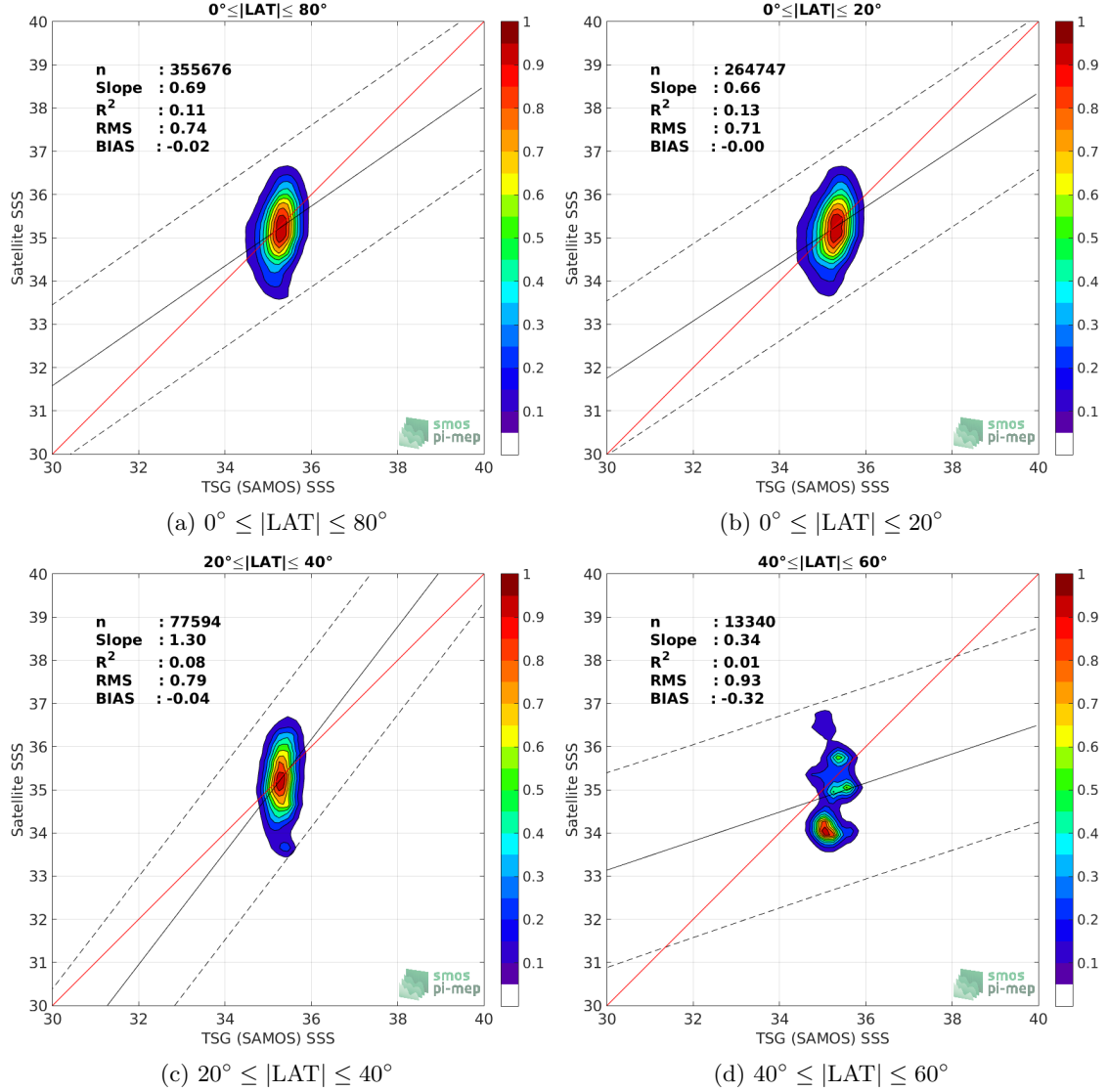
Figure 9: Contour maps of the concentration of SMOS SSS L2 v700 (ESA) SSS (y-axis) versus TSG (SAMOS) SSS (x-axis) at match-up pairs for different latitude bands. For each plot, the red line shows x=y . The black thin and dashed lines indicate a linear fit through the data cloud and the \pm 95\% confidence levels, respectively. The number match-up pairs n , the slope and R^2 coefficient of the linear fit, the root mean square (RMS) and the mean bias between satellite and in situ data are indicated for each latitude band in each plots.
