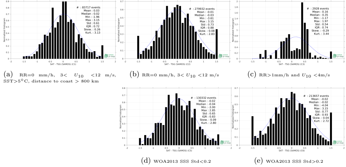
Figure 13: Normalized histogram of \Delta SSS (SMOS SSS L2 v700 (ESA) - TSG (SAMOS)) for 5 different subdatasets corresponding to: RR=0 mm/h, 3 < U_{10} < 12 m/s, SST>5°C, distance to coast > 800 km (a), RR=0 mm/h, 3 < U_{10} < 12 m/s (b), RR>1mm/h and U_{10} < 4 m/s (c), WOA2013 SSS Std<0.2 (d), WOA2013 SSS Std>0.2 (e).
