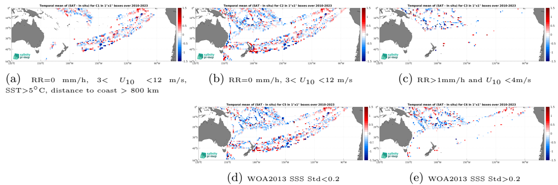
Figure 12: Temporal mean gridded over spatial boxes of size 1^\circ \times 1^\circ of \Delta\text{SSS} (SMOS SSS L2 v700 (ESA) - TSG (LEGOS-DM)) for 5 different subdatasets corresponding to: RR=0 mm/h, 3 < U_{10} < 12 m/s, SST > 5^\circ\text{C} , distance to coast > 800 km (a), RR=0 mm/h, 3 < U_{10} < 12 m/s (b), RR > 1\text{mm/h} and U_{10} < 4\text{m/s} (c), WOA2013 SSS Std < 0.2 (d), WOA2013 SSS Std > 0.2 (e).
