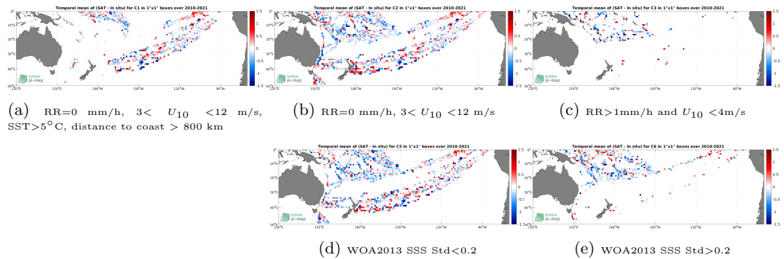
Figure 12: Temporal mean gridded over spatial boxes of size 1^\circ \times 1^\circ of \Delta SSS (SMOS SSS L2 v700 (ESA) - TSG (LEGOS-DM)) for 5 different subdatasets corresponding to:RR=0 mm/h, 3 < U_{10} < 12 m/s, SST >5^\circ\text{C} , distance to coast > 800 km (a), RR=0 mm/h, 3 < U_{10} < 12 m/s (b), RR >1 mm/h and U_{10} < 4 m/s (c), WOA2013 SSS Std <0.2 (d), WOA2013 SSS Std >0.2 (e).
