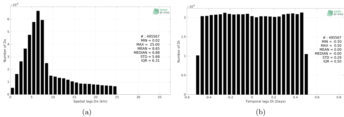
Figure 5: Histograms of the spatial (a) and temporal (b) lags between the location/time of the TSG (LEGOS-DM) measurement and the date of the corresponding SMOS SSS L2 v700 (ESA) SSS pixel.
