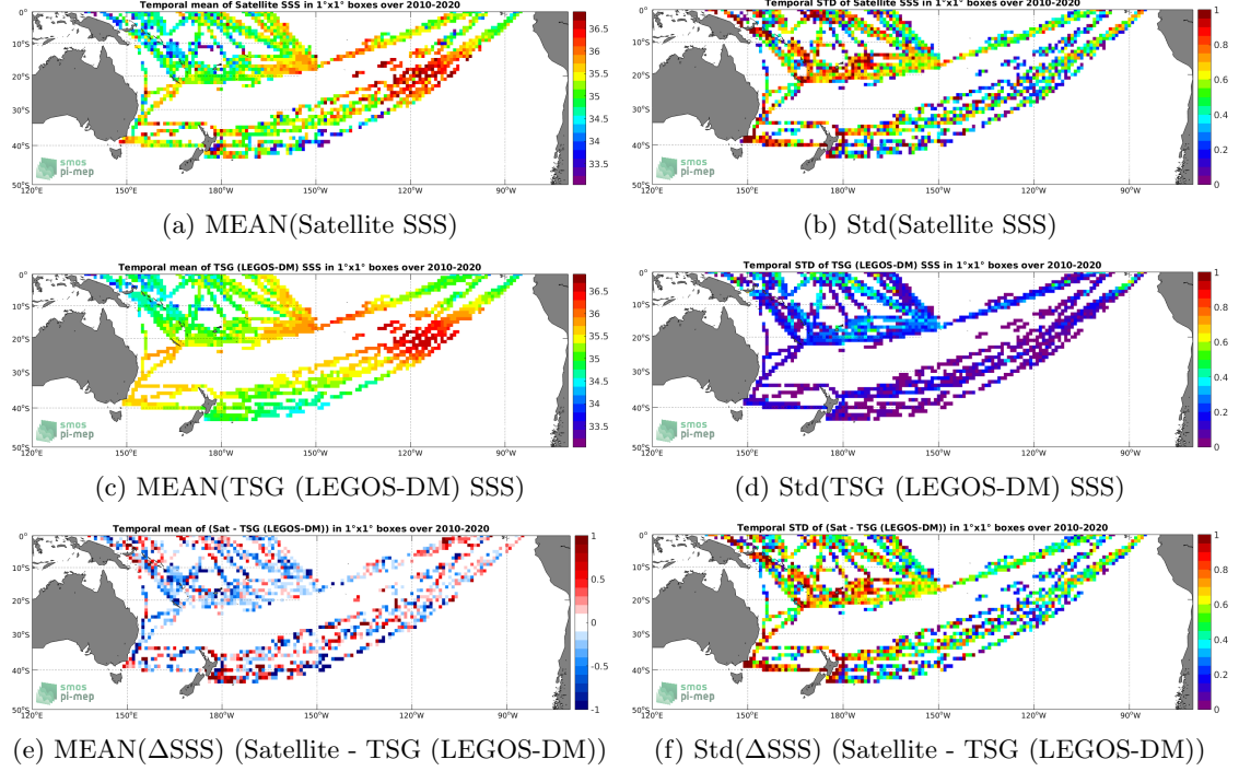
Figure 6: Temporal mean (left) and Std (right) of SSS from SMOS SSS L2 v700 (ESA) (top), TSG (LEGOS-DM) (middle), and of \Delta\text{SSS} (Satellite - TSG (LEGOS-DM)). Only match-up pairs are used to generate these maps.
