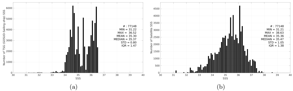
Figure 3: Histograms of SSS from TSG (GOSUD-Sailing-ship) (a) and SMOS SSS L2 v700 (ESA) (b) considering all match-up pairs per bins of 0.1 over the South Pacific Ocean Pi-MEP region and for the full satellite product period.
