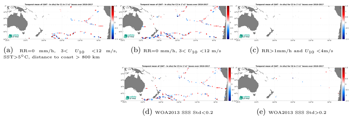
Figure 14: Temporal mean gridded over spatial boxes of size 1^\circ \times 1^\circ of \Delta SSS (SMOS SSS L2 v700 (ESA) - TSG (GOSUD-Sailing-ship)) for 5 different subdatasets corresponding to:RR=0 mm/h, 3 < U_{10} < 12 m/s, SST>5°C, distance to coast > 800 km (a), RR=0 mm/h, 3 < U_{10} < 12 m/s (b), RR>1mm/h and U_{10} < 4 m/s (c), WOA2013 SSS Std<0.2 (d), WOA2013 SSS Std>0.2 (e).
