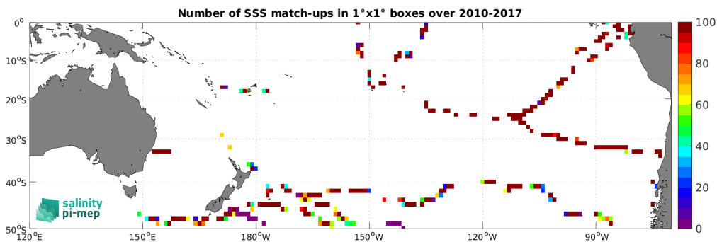
Figure 5: Number of SSS match-ups between TSG (GOSUD-Sailing-ship) SSS and the SMOS SSS L2 v700 (ESA) SSS product for the South Pacific Ocean Pi-MEP region over 1^\circ \times 1^\circ boxes and for the full satellite product period.
