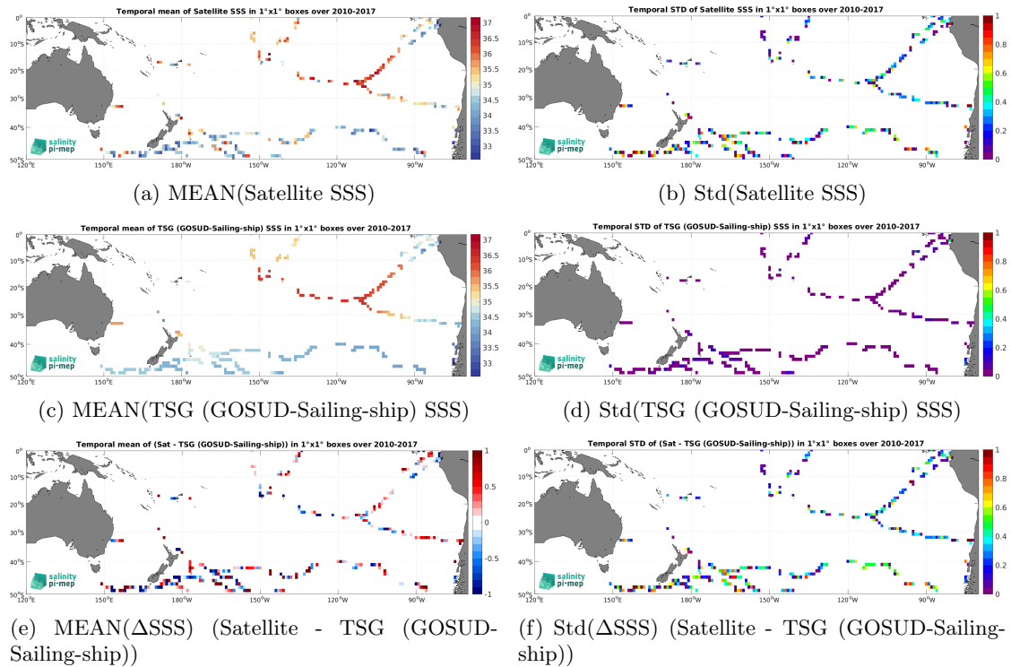
Figure 7: Temporal mean (left) and Std (right) of SSS from SMOS SSS L2 v700 (ESA) (top), TSG (GOSUD-Sailing-ship) (middle), and of \Delta SSS (Satellite - TSG (GOSUD-Sailing-ship)). Only match-up pairs are used to generate these maps.
