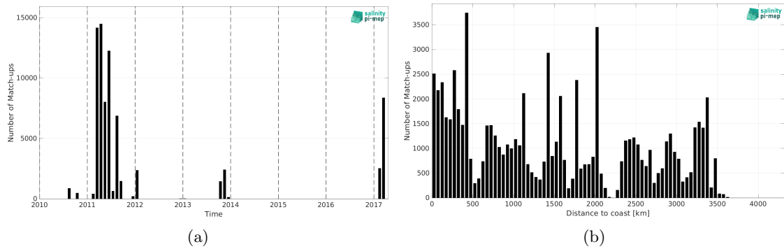
Figure 2: Number of match-ups between TSG (GOSUD-Sailing-ship) and SMOS SSS L2 v700 (ESA) SSS as a function of time (a) and as function of the distance to coast (b) over the South Pacific Ocean Pi-MEP region and for the full satellite product period.
