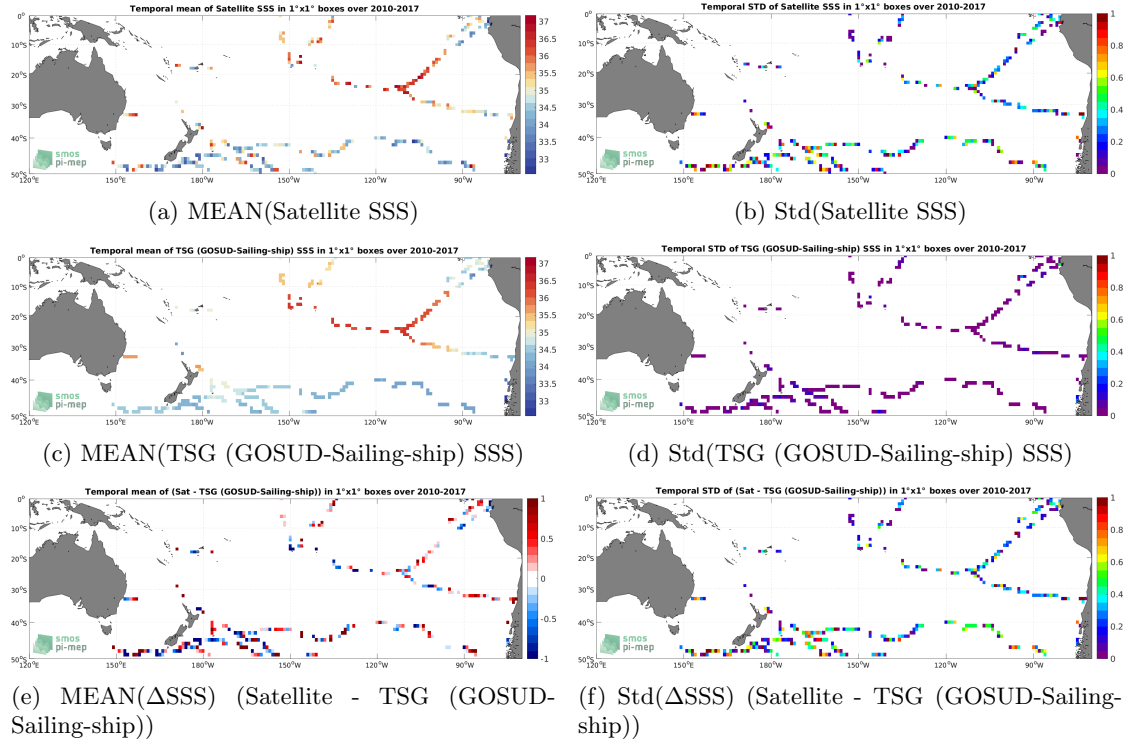
Figure 6: Temporal mean (left) and Std (right) of SSS from SMOS SSS L2 v700 (ESA) (top), TSG (GOSUD-Sailing-ship) (middle), and of \Delta SSS (Satellite - TSG (GOSUD-Sailing-ship)). Only match-up pairs are used to generate these maps.
