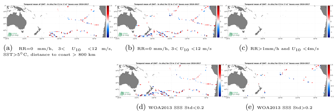
Figure 12: Temporal mean gridded over spatial boxes of size 1^\circ \times 1^\circ of \Delta SSS (SMOS SSS L2 v700 (ESA) - TSG (GOSUD-Sailing-ship)) for 5 different subdatasets corresponding to:RR=0 mm/h, 3 < U_{10} < 12 m/s, SST >5^\circ C, distance to coast > 800 km (a), RR=0 mm/h, 3 < U_{10} < 12 m/s (b), RR >1 mm/h and U_{10} < 4 m/s (c), WOA2013 SSS Std <0.2 (d), WOA2013 SSS Std >0.2 (e).
