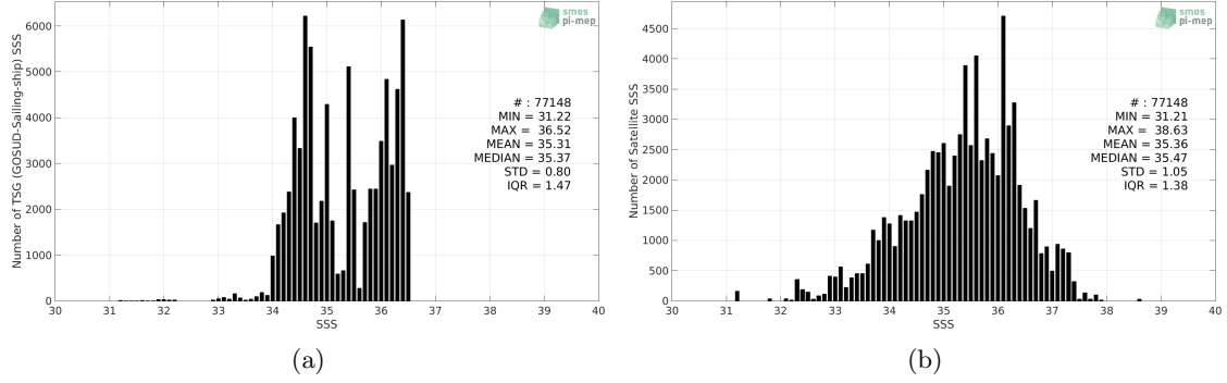
Figure 2: Histograms of SSS from TSG (GOSUD-Sailing-ship) (a) and SMOS SSS L2 v700 (ESA) (b) considering all match-up pairs per bins of 0.1 over the South Pacific Ocean Pi-MEP region and for the full satellite product period.
