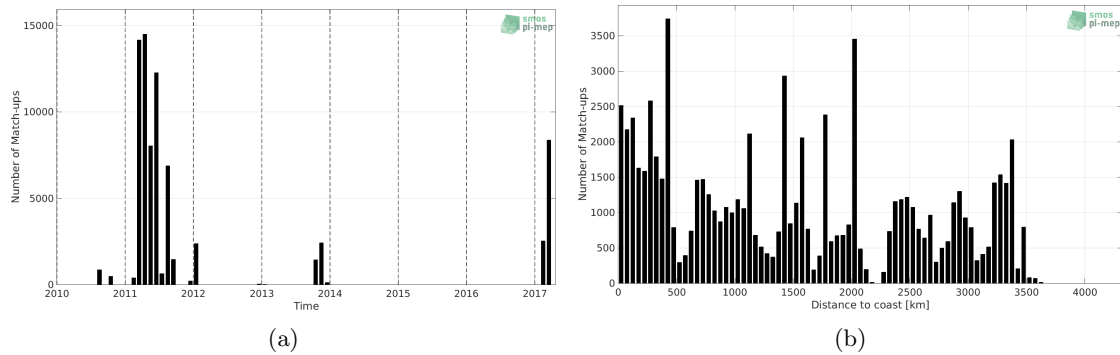
Figure 1: Number of match-ups between TSG (GOSUD-Sailing-ship) and SMOS SSS L2 v700 (ESA) SSS as a function of time (a) and as function of the distance to coast (b) over the South Pacific Ocean Pi-MEP region and for the full satellite product period.
