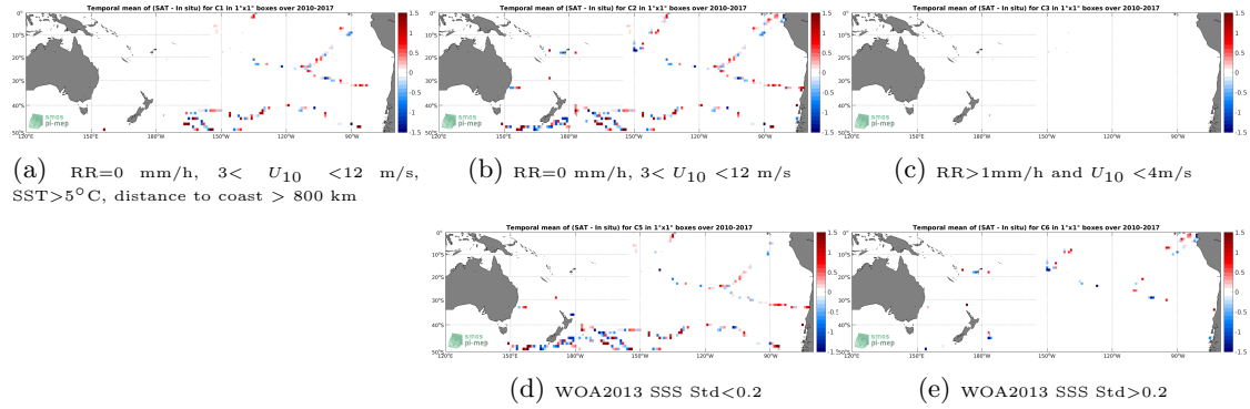
Figure 12: Temporal mean gridded over spatial boxes of size 1^\circ \times 1^\circ of \Delta SSS (SMOS SSS L2 v700 (ESA) - TSG (GOSUD-Sailing-ship)) for 5 different subdatasets corresponding to: RR=0 mm/h, 3 < U_{10} < 12 m/s, SST >5^\circ\text{C} , distance to coast > 800 km (a), RR=0 mm/h, 3 < U_{10} < 12 m/s (b), RR>1\text{mm/h} and U_{10} < 4\text{m/s} (c), WOA2013 SSS Std <0.2 (d), WOA2013 SSS Std >0.2 (e).
