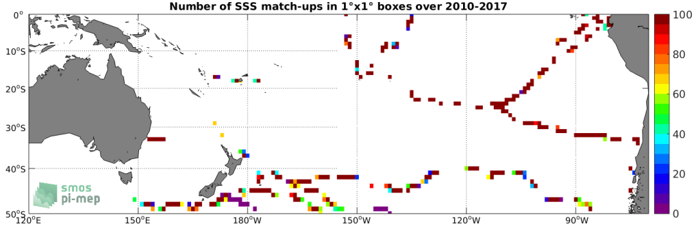
Figure 4: Number of SSS match-ups between TSG (GOSUD-Sailing-ship) SSS and the SMOS SSS L2 v700 (ESA) SSS product for the South Pacific Ocean Pi-MEP region over 1^\circ \times 1^\circ boxes and for the full satellite product period.
