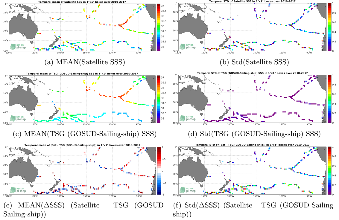
Figure 6: Temporal mean (left) and Std (right) of SSS from SMOS SSS L2 v700 (ESA) (top), TSG (GOSUD-Sailing-ship) (middle), and of \Delta SSS (Satellite - TSG (GOSUD-Sailing-ship)). Only match-up pairs are used to generate these maps.
