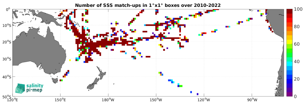
Figure 5: Number of SSS match-ups between TSG (GOSUD-Research-vessel) SSS and the SMOS SSS L2 v700 (ESA) SSS product for the South Pacific Ocean Pi-MEP region over 1^\circ \times 1^\circ boxes and for the full satellite product period.
