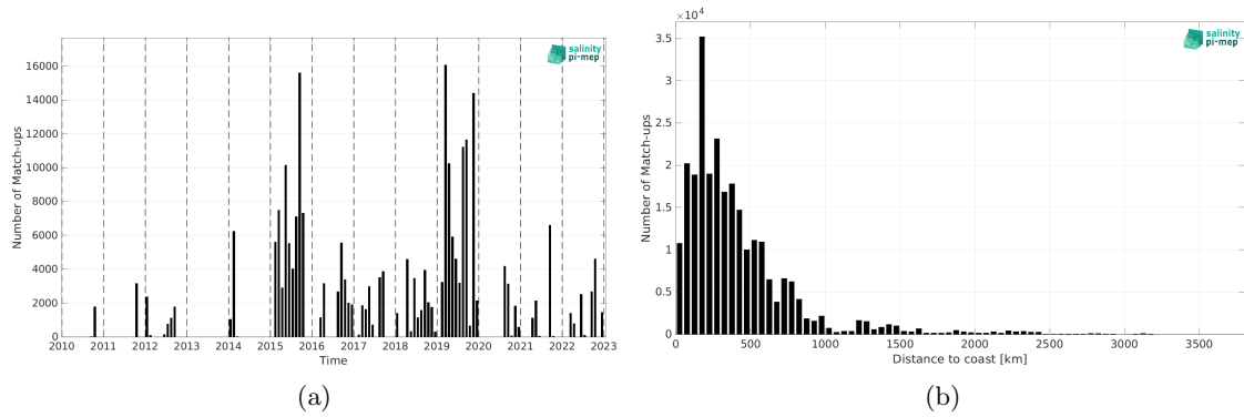
Figure 2: Number of match-ups between TSG (GOSUD-Research-vessel) and SMOS SSS L2 v700 (ESA) SSS as a function of time (a) and as function of the distance to coast (b) over the South Pacific Ocean Pi-MEP region and for the full satellite product period.
