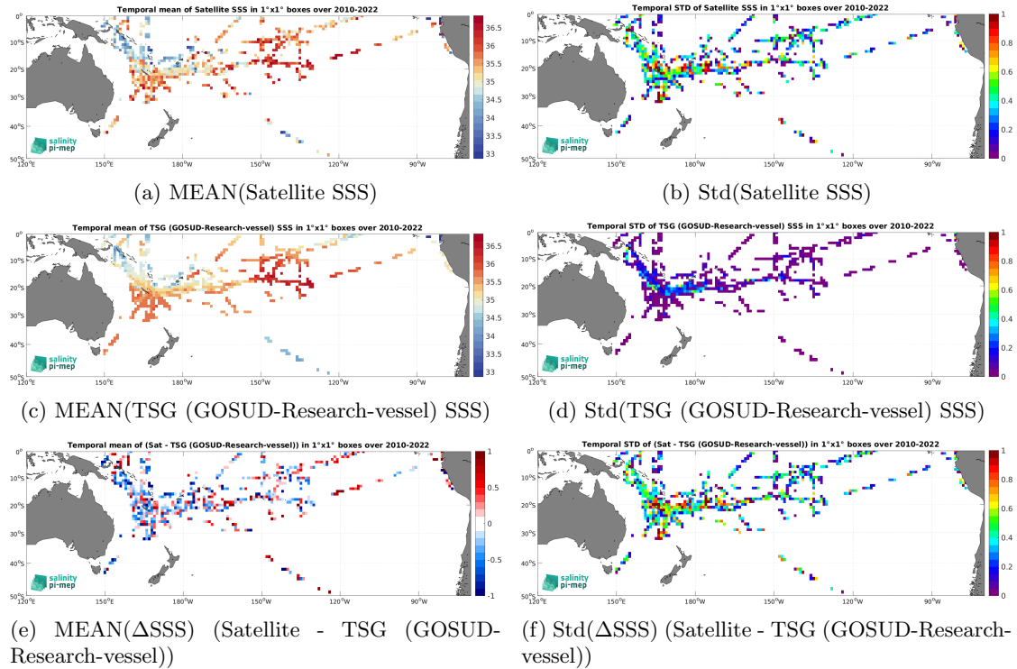
Figure 7: Temporal mean (left) and Std (right) of SSS from SMOS SSS L2 v700 (ESA) (top), TSG (GOSUD-Research-vessel) (middle), and of \Delta SSS (Satellite - TSG (GOSUD-Research-vessel)). Only match-up pairs are used to generate these maps.
