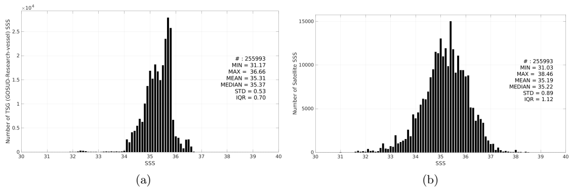
Figure 3: Histograms of SSS from TSG (GOSUD-Research-vessel) (a) and SMOS SSS L2 v700 (ESA) (b) considering all match-up pairs per bins of 0.1 over the South Pacific Ocean Pi-MEP region and for the full satellite product period.
