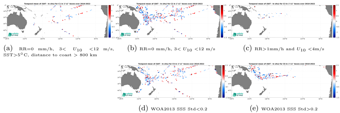
Figure 14: Temporal mean gridded over spatial boxes of size 1^\circ \times 1^\circ of \Delta SSS (SMOS SSS L2 v700 (ESA) - TSG (GOSUD-Research-vessel)) for 5 different subdatasets corresponding to:RR=0 mm/h, 3 < U_{10} < 12 m/s, SST>5°C, distance to coast > 800 km (a), RR=0 mm/h, 3 < U_{10} < 12 m/s (b), RR>1mm/h and U_{10} < 4 m/s (c), WOA2013 SSS Std<0.2 (d), WOA2013 SSS Std>0.2 (e).
