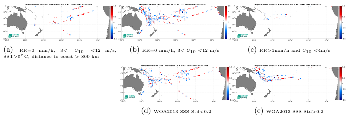
Figure 12: Temporal mean gridded over spatial boxes of size 1^\circ \times 1^\circ of \Delta\text{SSS} (SMOS SSS L2 v700 (ESA) - TSG (GOSUD-Research-vessel)) for 5 different subdatasets corresponding to:RR=0 mm/h, 3 < U_{10} < 12 m/s, SST>5°C, distance to coast > 800 km (a), RR=0 mm/h, 3 < U_{10} < 12 m/s (b), RR>1mm/h and U_{10} < 4 m/s (c), WOA2013 SSS Std<0.2 (d), WOA2013 SSS Std>0.2 (e).
