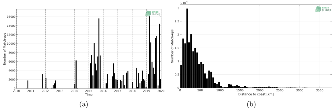
Figure 1: Number of match-ups between TSG (GOSUD-Research-vessel) and SMOS SSS L2 v700 (ESA) SSS as a function of time (a) and as function of the distance to coast (b) over the South Pacific Ocean Pi-MEP region and for the full satellite product period.
