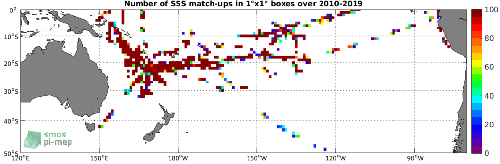
Figure 4: Number of SSS match-ups between TSG (GOSUD-Research-vessel) SSS and the SMOS SSS L2 v700 (ESA) SSS product for the South Pacific Ocean Pi-MEP region over 1^\circ \times 1^\circ boxes and for the full satellite product period.
