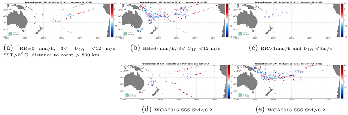
Figure 12: Temporal mean gridded over spatial boxes of size 1^\circ \times 1^\circ of \Delta SSS (SMOS SSS L2 v700 (ESA) - TSG (GOSUD-Research-vessel)) for 5 different subdatasets corresponding to: RR=0 mm/h, 3 < U_{10} < 12 m/s, SST >5^\circ C, distance to coast > 800 km (a), RR=0 mm/h, 3 < U_{10} < 12 m/s (b), RR>1 mm/h and U_{10} < 4 m/s (c), WOA2013 SSS Std <0.2 (d), WOA2013 SSS Std >0.2 (e).
