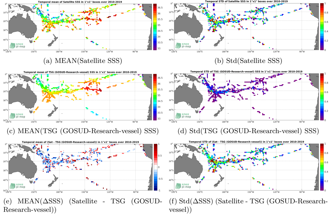
Figure 6: Temporal mean (left) and Std (right) of SSS from SMOS SSS L2 v700 (ESA) (top), TSG (GOSUD-Research-vessel) (middle), and of \Delta SSS (Satellite - TSG (GOSUD-Research-vessel)). Only match-up pairs are used to generate these maps.
