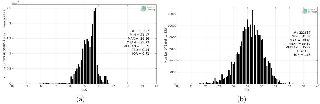
Figure 2: Histograms of SSS from TSG (GOSUD-Research-vessel) (a) and SMOS SSS L2 v700 (ESA) (b) considering all match-up pairs per bins of 0.1 over the South Pacific Ocean Pi-MEP region and for the full satellite product period.
