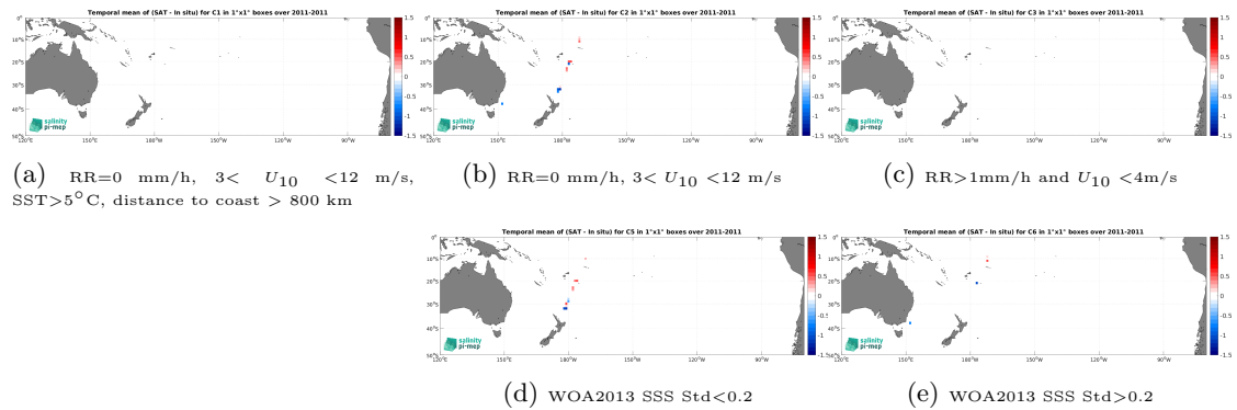
Figure 12: Temporal mean gridded over spatial boxes of size 1^\circ \times 1^\circ of \Delta SSS (SMOS SSS L2 v700 (ESA) - TSG (CSIC-UTM)) for 5 different subdatasets corresponding to:RR=0 mm/h, 3 < U_{10} < 12 m/s, SST >5^\circ C, distance to coast > 800 km (a), RR=0 mm/h, 3 < U_{10} < 12 m/s (b), RR >1 mm/h and U_{10} < 4 m/s (c), WOA2013 SSS Std <0.2 (d), WOA2013 SSS Std >0.2 (e).
