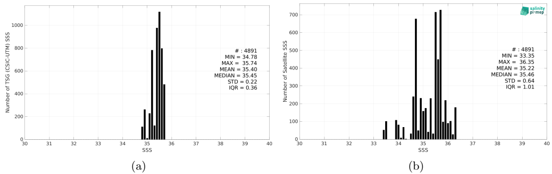
Figure 2: Histograms of SSS from TSG (CSIC-UTM) (a) and SMOS SSS L2 v700 (ESA) (b) considering all match-up pairs per bins of 0.1 over the South Pacific Ocean Pi-MEP region and for the full satellite product period.
