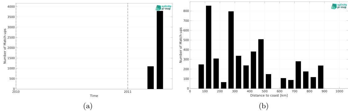
Figure 1: Number of match-ups between TSG (CSIC-UTM) and SMOS SSS L2 v700 (ESA) SSS as a function of time (a) and as function of the distance to coast (b) over the South Pacific Ocean Pi-MEP region and for the full satellite product period.
