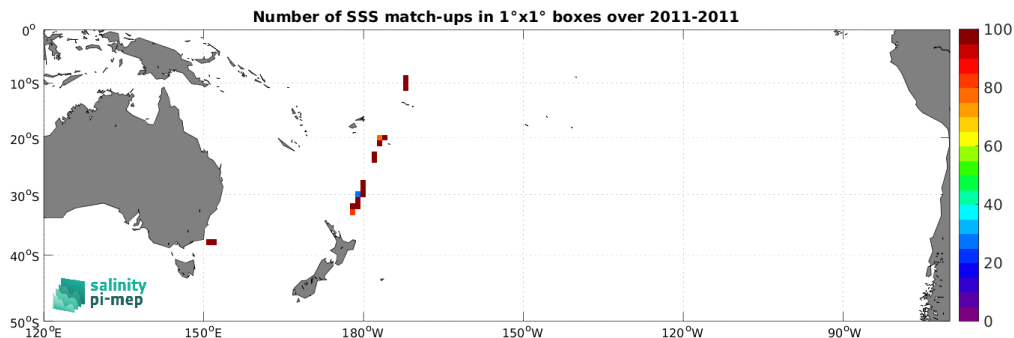
Figure 4: Number of SSS match-ups between TSG (CSIC-UTM) SSS and the SMOS SSS L2 v700 (ESA) SSS product for the South Pacific Ocean Pi-MEP region over 1^\circ \times 1^\circ boxes and for the full satellite product period.
