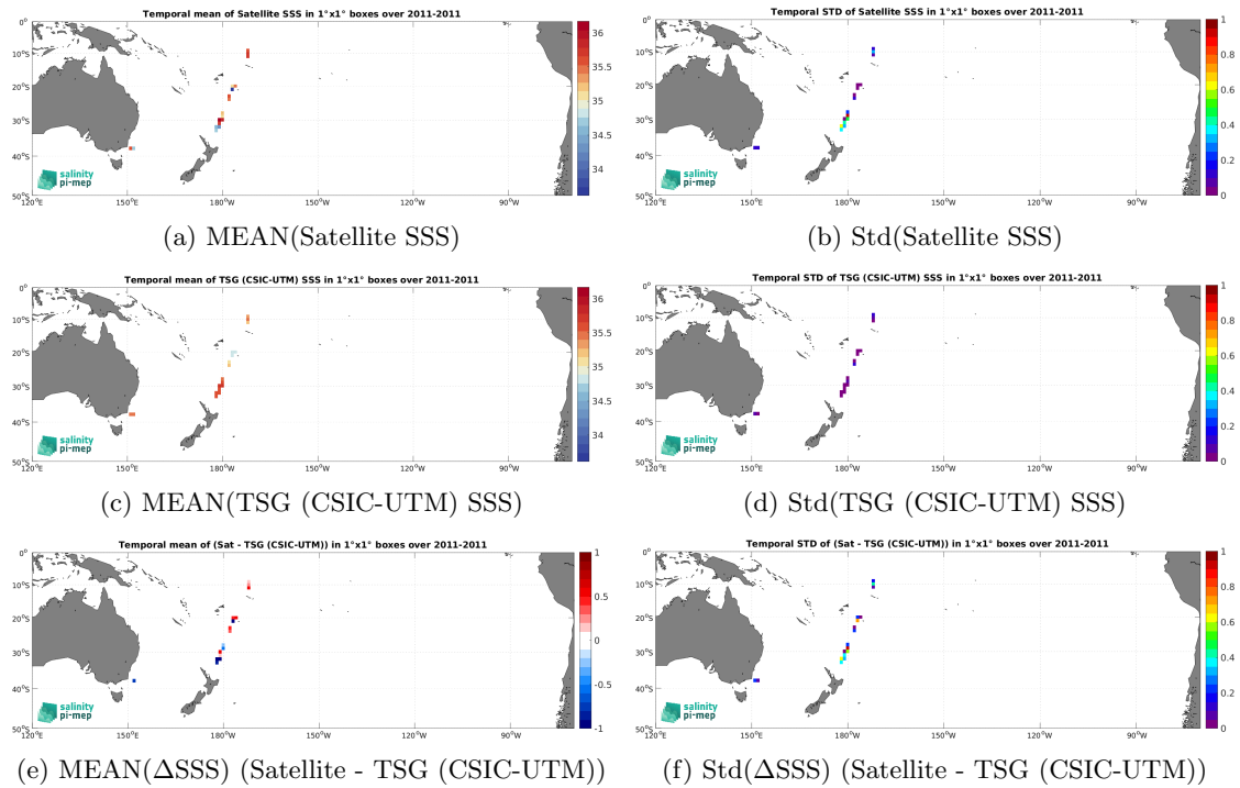
Figure 6: Temporal mean (left) and Std (right) of SSS from SMOS SSS L2 v700 (ESA) (top), TSG (CSIC-UTM) (middle), and of \Delta SSS (Satellite - TSG (CSIC-UTM)). Only match-up pairs are used to generate these maps.
