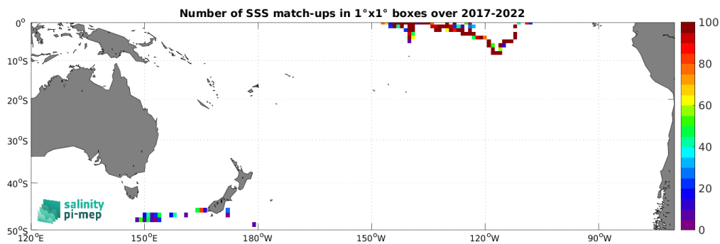
Figure 5: Number of SSS match-ups between Saildrone SSS and the SMOS SSS L2 v700 (ESA) SSS product for the South Pacific Ocean Pi-MEP region over 1^\circ \times 1^\circ boxes and for the full satellite product period.
