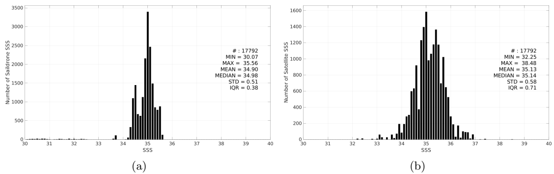
Figure 3: Histograms of SSS from Saildrone (a) and SMOS SSS L2 v700 (ESA) (b) considering all match-up pairs per bins of 0.1 over the South Pacific Ocean Pi-MEP region and for the full satellite product period.
