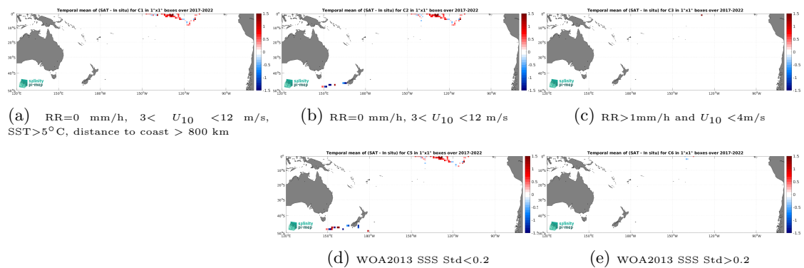
Figure 14: Temporal mean gridded over spatial boxes of size 1^\circ \times 1^\circ of \Delta SSS (SMOS SSS L2 v700 (ESA) - Sairdrone) for 5 different subdatasets corresponding to:RR=0 mm/h, 3 < U_{10} < 12 m/s, SST >5^\circ C, distance to coast > 800 km (a), RR=0 mm/h, 3 < U_{10} < 12 m/s (b), RR >1 mm/h and U_{10} < 4 m/s (c), WOA2013 SSS Std <0.2 (d), WOA2013 SSS Std >0.2 (e).
