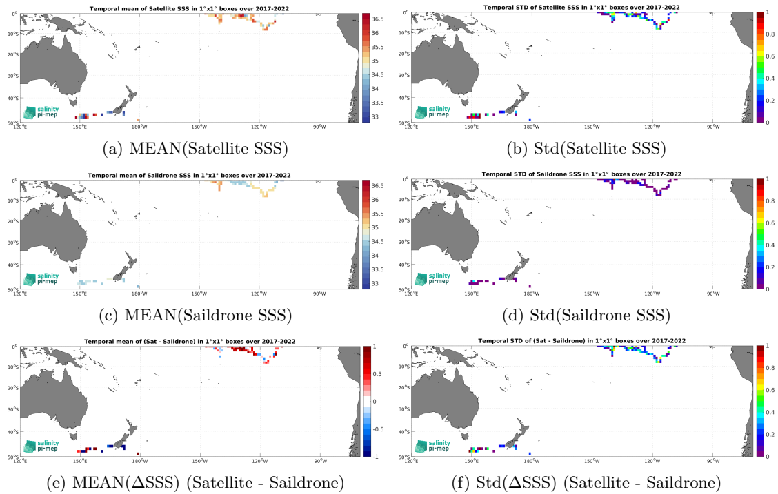
Figure 7: Temporal mean (left) and Std (right) of SSS from SMOS SSS L2 v700 (ESA) (top), Saildrone (middle), and of \Delta SSS (Satellite - Saildrone). Only match-up pairs are used to generate these maps.
