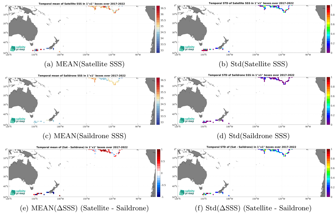
Figure 6: Temporal mean (left) and Std (right) of SSS from SMOS SSS L2 v700 (ESA) (top), Saildrone (middle), and of \Delta SSS (Satellite - Saildrone). Only match-up pairs are used to generate these maps.
