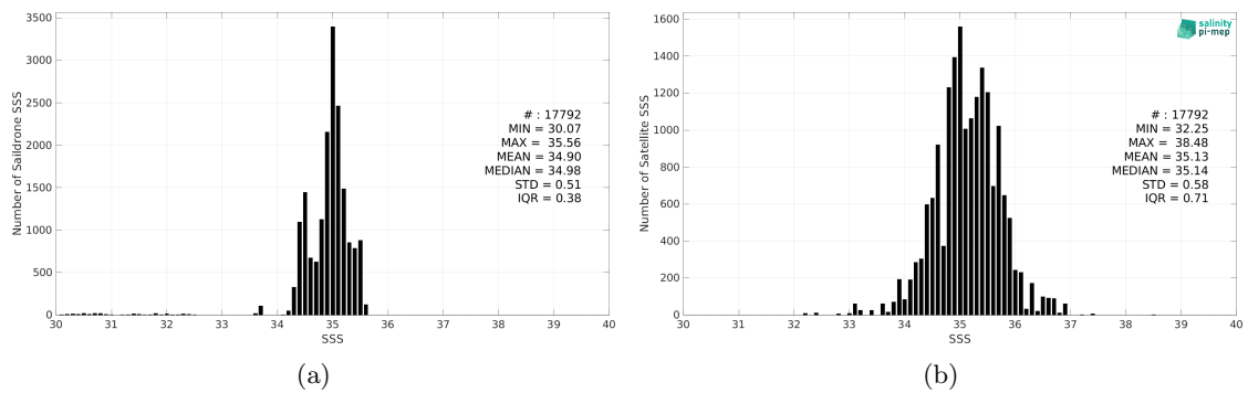
Figure 2: Histograms of SSS from Saildrone (a) and SMOS SSS L2 v700 (ESA) (b) considering all match-up pairs per bins of 0.1 over the South Pacific Ocean Pi-MEP region and for the full satellite product period.
