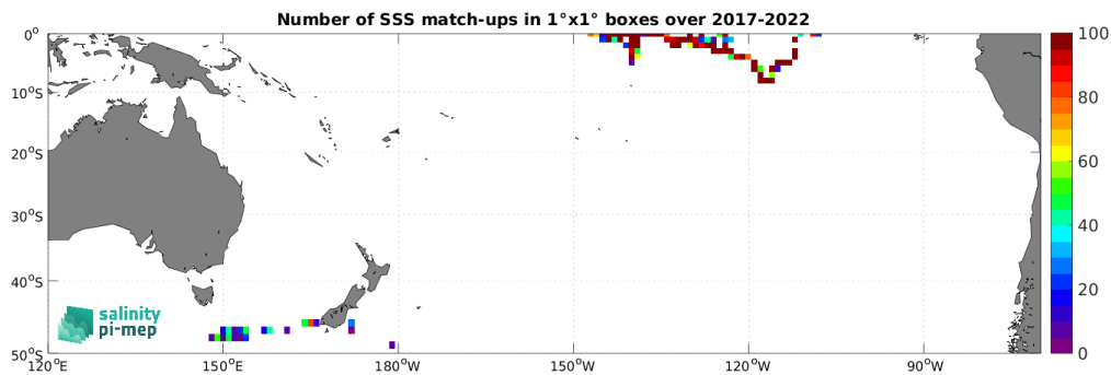
Figure 4: Number of SSS match-ups between Saildrone SSS and the SMOS SSS L2 v700 (ESA) SSS product for the South Pacific Ocean Pi-MEP region over 1^\circ \times 1^\circ boxes and for the full satellite product period.
