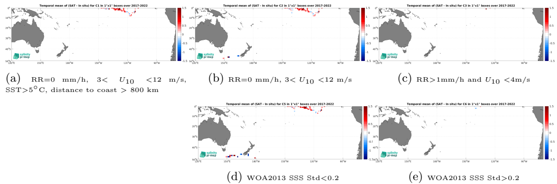
Figure 12: Temporal mean gridded over spatial boxes of size 1^\circ \times 1^\circ of \Delta SSS (SMOS SSS L2 v700 (ESA) - Sairdrone) for 5 different subdatasets corresponding to:RR=0 mm/h, 3 < U_{10} < 12 m/s, SST >5^\circ C, distance to coast > 800 km (a), RR=0 mm/h, 3 < U_{10} < 12 m/s (b), RR >1 mm/h and U_{10} < 4 m/s (c), WOA2013 SSS Std <0.2 (d), WOA2013 SSS Std >0.2 (e).
