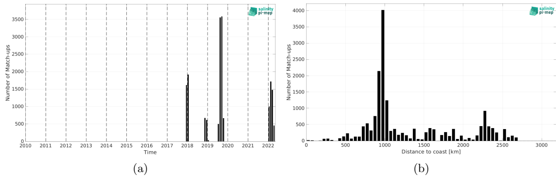
Figure 1: Number of match-ups between Saildrone and SMOS SSS L2 v700 (ESA) SSS as a function of time (a) and as function of the distance to coast (b) over the South Pacific Ocean Pi-MEP region and for the full satellite product period.
