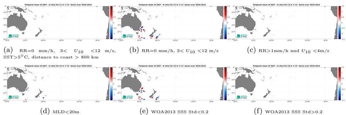
Figure 12: Temporal mean gridded over spatial boxes of size 1^\circ \times 1^\circ of \Delta SSS (SMOS SSS L2 v700 (ESA) - Marine mammals) for 6 different subdatasets corresponding to:RR=0 mm/h, 3 < U_{10} < 12 m/s, SST >5^\circ C, distance to coast > 800 km (a), RR=0 mm/h, 3 < U_{10} < 12 m/s (b), RR >1 mm/h and U_{10} < 4 m/s (c),MLD <20 m (d),WOA2013 SSS Std <0.2 (e),WOA2013 SSS Std >0.2 (f).
