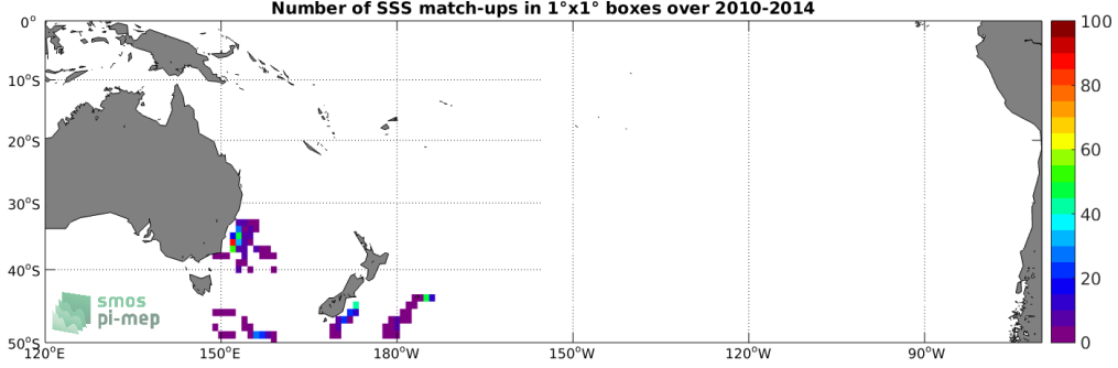
Figure 4: Number of SSS match-ups between Marine mammals SSS and the SMOS SSS L2 v700 (ESA) SSS product for the South Pacific Ocean Pi-MEP region over 1^\circ \times 1^\circ boxes and for the full satellite product period.
