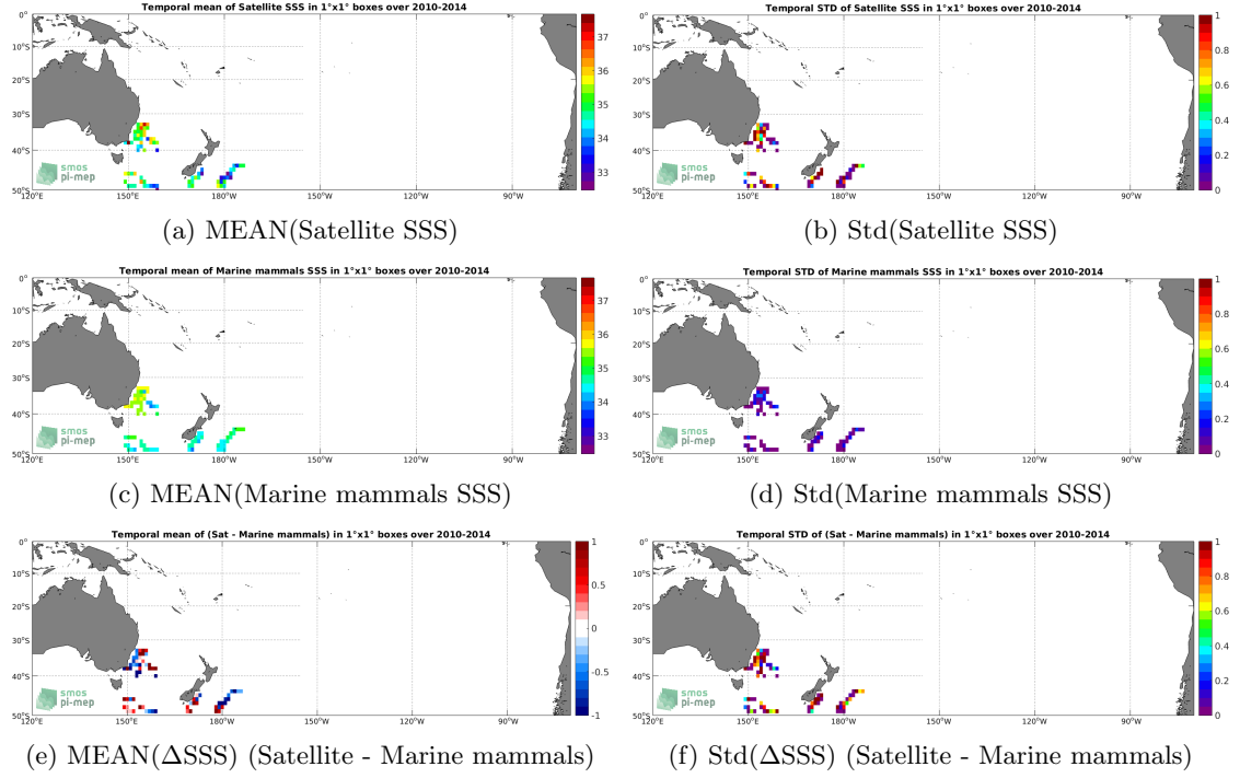
Figure 6: Temporal mean (left) and Std (right) of SSS from SMOS SSS L2 v700 (ESA) (top), Marine mammals (middle), and of \Delta SSS (Satellite - Marine mammals). Only match-up pairs are used to generate these maps.
