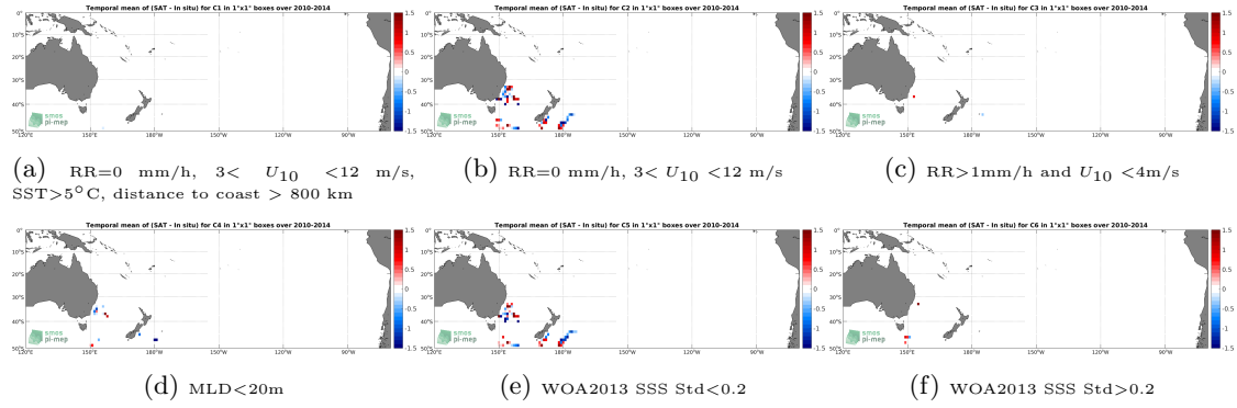
Figure 12: Temporal mean gridded over spatial boxes of size 1^\circ \times 1^\circ of \Delta SSS (SMOS SSS L2 v700 (ESA) - Marine mammals) for 6 different subdatasets corresponding to: RR=0 mm/h, 3 < U_{10} < 12 m/s, SST > 5^\circ C , distance to coast > 800 km (a), RR=0 mm/h, 3 < U_{10} < 12 m/s (b), RR > 1 mm/h and U_{10} < 4 m/s (c), MLD < 20 m (d), WOA2013 SSS Std < 0.2 (e), WOA2013 SSS Std > 0.2 (f).
