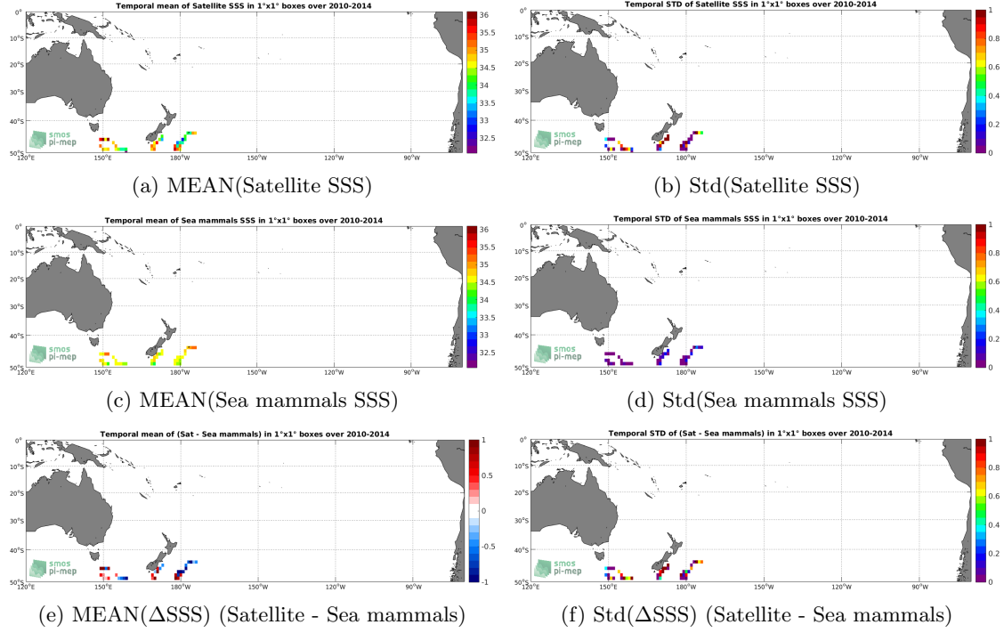
Figure 6: Temporal mean (left) and Std (right) of SSS from SMOS SSS L2 v700 (ESA) (top), Sea mammals (middle), and of \Delta SSS (Satellite - Sea mammals). Only match-up pairs are used to generate these maps.
