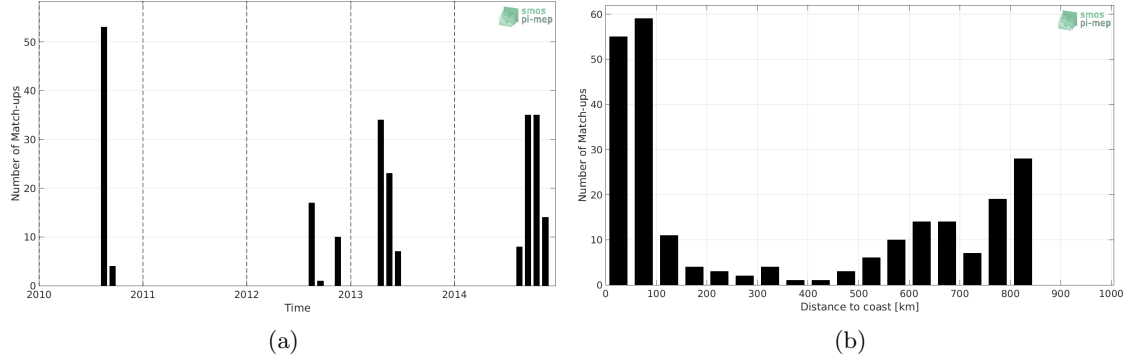
Figure 1: Number of match-ups between Sea mammals and SMOS SSS L2 v700 (ESA) SSS as a function of time (a) and as function of the distance to coast (b) over the South Pacific Ocean Pi-MEP region and for the full satellite product period.
