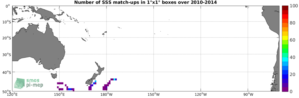
Figure 4: Number of SSS match-ups between Sea mammals SSS and the SMOS SSS L2 v700 (ESA) SSS product for the South Pacific Ocean Pi-MEP region over 1^\circ \times 1^\circ boxes and for the full satellite product period.
