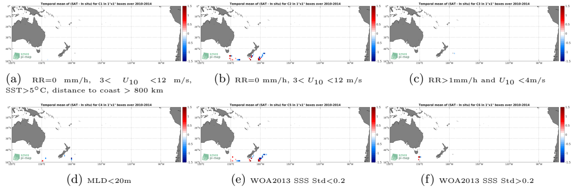
Figure 12: Temporal mean gridded over spatial boxes of size 1^{\circ}\times 1^{\circ} of \Delta\text{SSS} (SMOS SSS L2 v700 (ESA) - Sea mammals) for 6 different subdatasets corresponding to: \text{RR}=0 mm/h, 3 < U_{10} < 12 m/s, \text{SST} > 5^{\circ}\text{C} , distance to coast > 800 km (a), \text{RR}=0 mm/h, 3 < U_{10} < 12 m/s (b), \text{RR} > 1\text{mm/h} and U_{10} < 4\text{m/s} (c), \text{MLD} < 20\text{m} (d), \text{WOA2013 SSS Std} < 0.2 (e), \text{WOA2013 SSS Std} > 0.2 (f).
