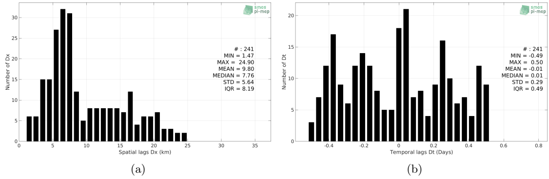
Figure 5: Histograms of the spatial (a) and temporal (b) lags between the location/time of the Sea mammals measurement and the date of the corresponding SMOS SSS L2 v700 (ESA) SSS pixel.
