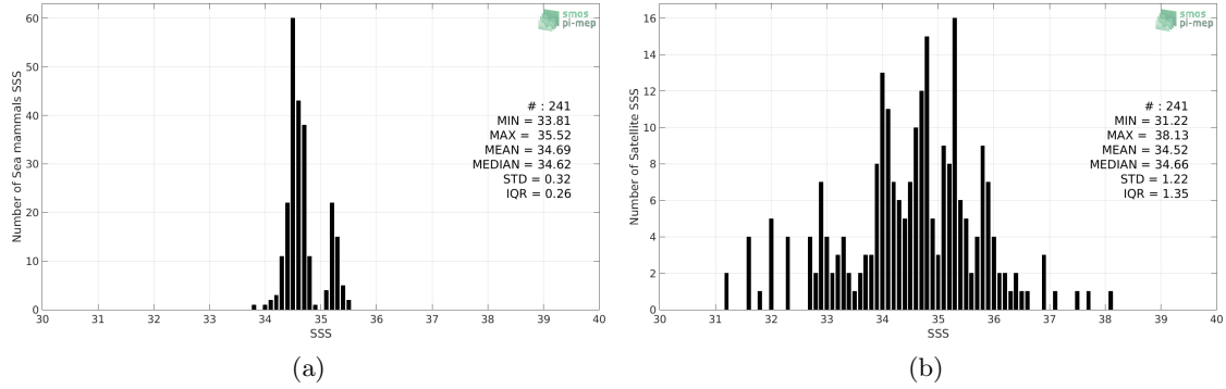
Figure 2: Histograms of SSS from Sea mammals (a) and SMOS SSS L2 v700 (ESA) (b) considering all match-up pairs per bins of 0.1 over the South Pacific Ocean Pi-MEP region and for the full satellite product period.
