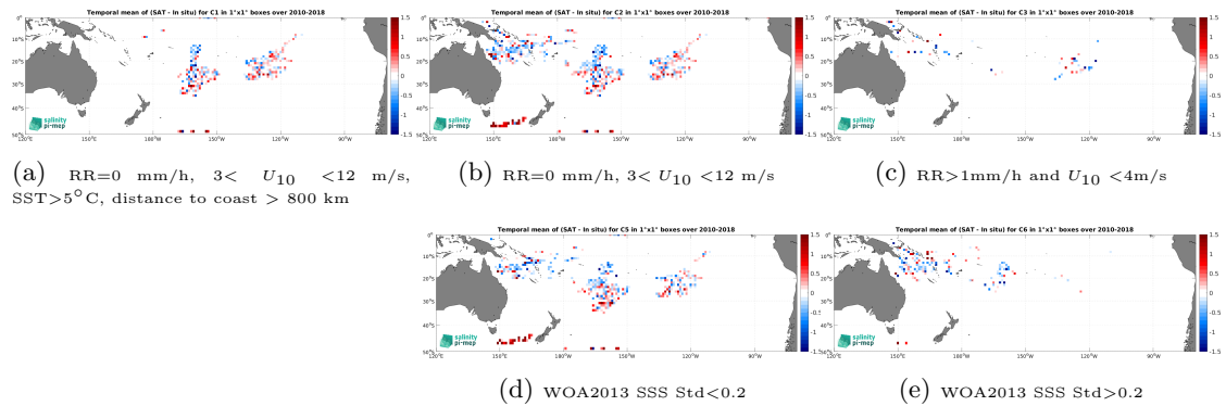
Figure 13: Temporal mean gridded over spatial boxes of size 1^\circ \times 1^\circ of \Delta\text{SSS} (SMOS SSS L2 v700 (ESA) - Surface drifters) for 5 different subdatasets corresponding to:RR=0 mm/h, 3 < U_{10} < 12 m/s, SST >5^\circ\text{C} , distance to coast > 800 km (a), RR=0 mm/h, 3 < U_{10} < 12 m/s (b), RR >1 mm/h and U_{10} < 4 m/s (c), WOA2013 SSS Std <0.2 (d), WOA2013 SSS Std >0.2 (e).
