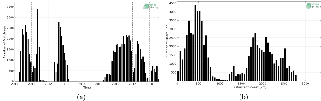
Figure 1: Number of match-ups between Surface drifters and SMOS SSS L2 v700 (ESA) SSS as a function of time (a) and as function of the distance to coast (b) over the South Pacific Ocean Pi-MEP region and for the full satellite product period.
