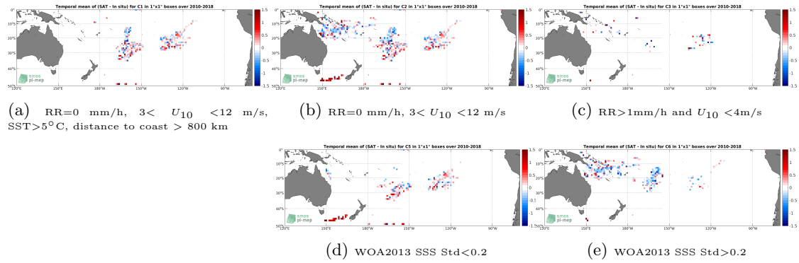
Figure 11: Temporal mean gridded over spatial boxes of size 1^\circ \times 1^\circ of \Delta SSS (SMOS SSS L2 v700 (ESA) - Surface drifters) for 5 different subdatasets corresponding to: RR=0 mm/h, 3 < U_{10} < 12 m/s, SST >5^\circ\text{C} , distance to coast > 800 km (a), RR=0 mm/h, 3 < U_{10} < 12 m/s (b), RR>1\text{mm/h} and U_{10} < 4\text{m/s} (c), WOA2013 SSS Std <0.2 (d), WOA2013 SSS Std >0.2 (e).
