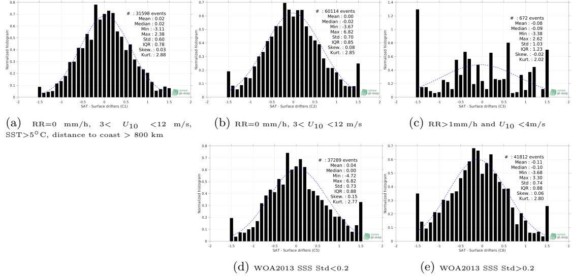
Figure 12: Normalized histogram of \Delta\text{SSS} (SMOS SSS L2 v700 (ESA) - Surface drifters) for 5 different subdatasets corresponding to: RR=0 mm/h, 3 < U_{10} < 12 m/s, SST>5°C, distance to coast > 800 km (a), RR=0 mm/h, 3 < U_{10} < 12 m/s (b), RR>1mm/h and U_{10} < 4 m/s (c), WOA2013 SSS Std<0.2 (d), WOA2013 SSS Std>0.2 (e).
