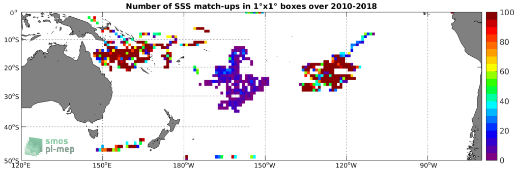
Figure 3: Number of SSS match-ups between Surface drifters SSS and the SMOS SSS L2 v700 (ESA) SSS product for the South Pacific Ocean Pi-MEP region over 1^\circ \times 1^\circ boxes and for the full satellite product period.
