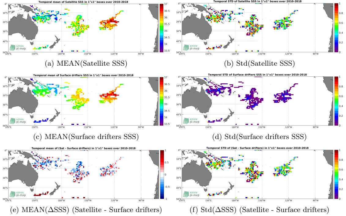
Figure 5: Temporal mean (left) and Std (right) of SSS from SMOS SSS L2 v700 (ESA) (top), Surface drifters (middle), and of \Delta SSS (Satellite - Surface drifters). Only match-up pairs are used to generate these maps.
