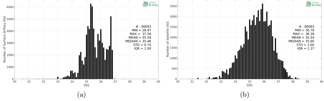
Figure 2: Histograms of SSS from Surface drifters (a) and SMOS SSS L2 v700 (ESA) (b) considering all match-up pairs per bins of 0.1 over the South Pacific Ocean Pi-MEP region and for the full satellite product period.
