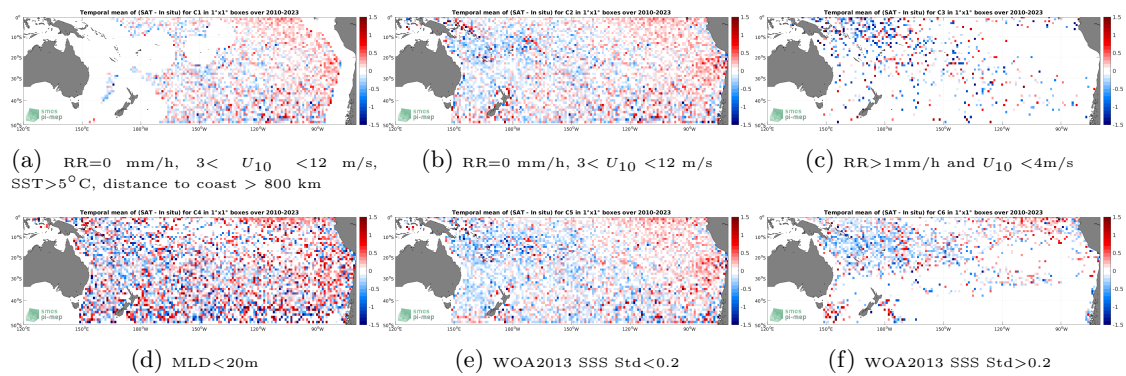
Figure 12: Temporal mean gridded over spatial boxes of size 1^\circ \times 1^\circ of \Delta SSS (SMOS SSS L2 v700 (ESA) - Argo) for 6 different subdatasets corresponding to:RR=0 mm/h, 3 < U_{10} < 12 m/s, SST >5^\circ\text{C} , distance to coast > 800 km (a), RR=0 mm/h, 3 < U_{10} < 12 m/s (b), RR >1 mm/h and U_{10} < 4 m/s (c),MLD <20 m (d),WOA2013 SSS Std <0.2 (e),WOA2013 SSS Std >0.2 (f).
