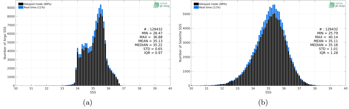
Figure 2: Histograms of SSS from Argo (a) and SMOS SSS L2 v700 (ESA) (b) considering all match-up pairs per bins of 0.1 over the South Pacific Ocean Pi-MEP region and for the full satellite product period.
