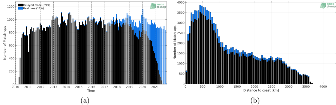
Figure 1: Number of match-ups between Argo and SMOS SSS L2 v700 (ESA) SSS as a function of time (a) and as function of the distance to coast (b) over the South Pacific Ocean Pi-MEP region and for the full satellite product period.
