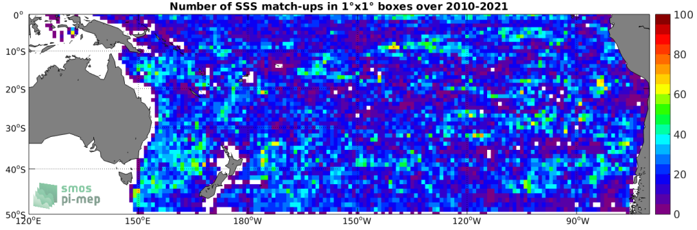
Figure 4: Number of SSS match-ups between Argo SSS and the SMOS SSS L2 v700 (ESA) SSS product for the South Pacific Ocean Pi-MEP region over 1^\circ \times 1^\circ boxes and for the full satellite product period.
