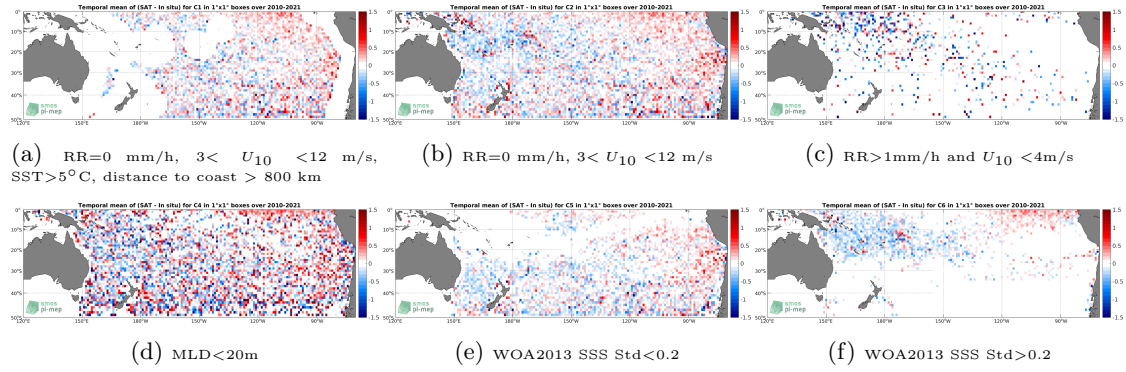
Figure 12: Temporal mean gridded over spatial boxes of size 1^\circ \times 1^\circ of \Delta SSS (SMOS SSS L2 v700 (ESA) - Argo) for 6 different subdatasets corresponding to: RR=0 mm/h, 3 < U_{10} < 12 m/s, SST > 5^\circ C , distance to coast > 800 km (a), RR=0 mm/h, 3 < U_{10} < 12 m/s (b), RR > 1 mm/h and U_{10} < 4 m/s (c), MLD < 20 m (d), WOA2013 SSS Std < 0.2 (e), WOA2013 SSS Std > 0.2 (f).
