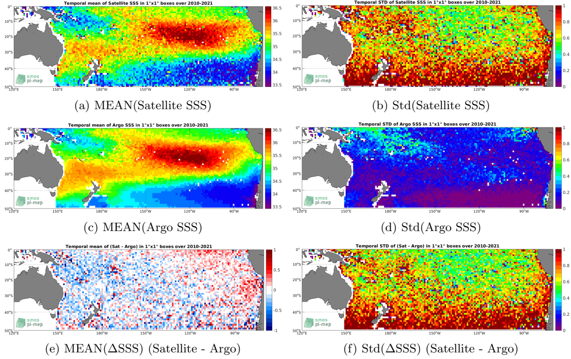
Figure 6: Temporal mean (left) and Std (right) of SSS from SMOS SSS L2 v700 (ESA) (top), Argo (middle), and of \Delta SSS (Satellite - Argo). Only match-up pairs are used to generate these maps.
